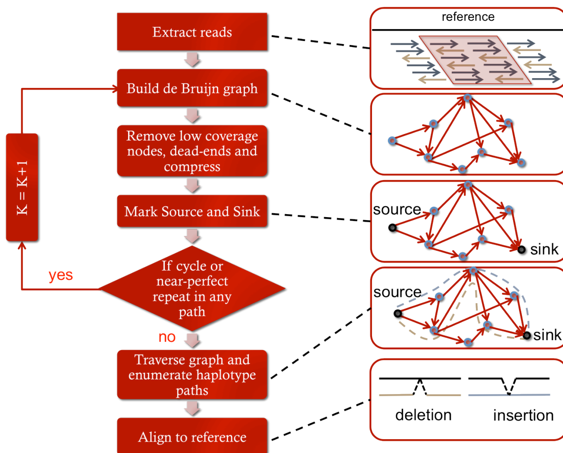
Figure 1. Overview of the Scalpel algorithm workflow.
