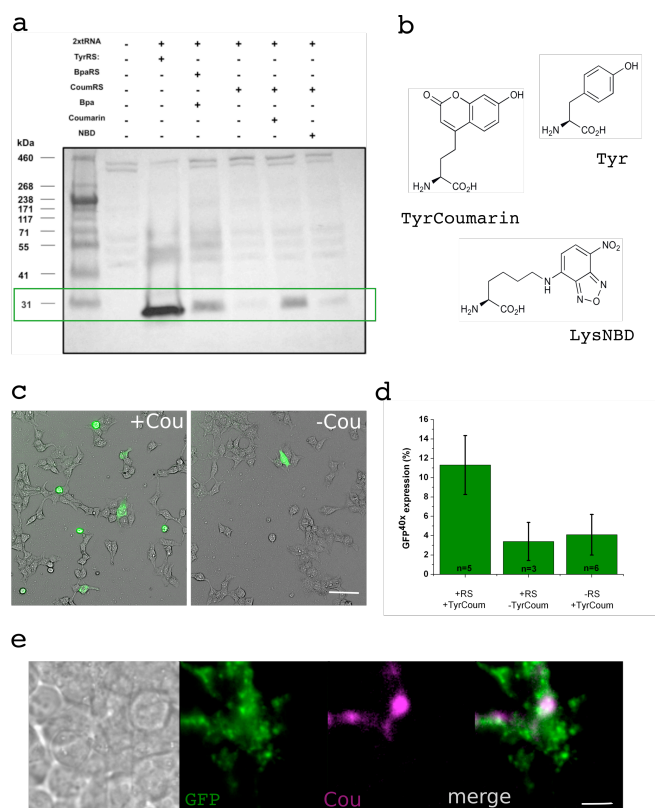
Figure 2: Amber codon suppression and incorporation of a coumarinyl amino acid in HEK-293T cells. (a) Western blots for the detection of amber suppression in HEK-293T cells expressing the GFP 40 TAG gene in the absence or presence of Tyr-coumarin and Lys-NBD (lower band at 30 kDa, green box). 2 nd lane is transfected with GFP 40 TAG alone and the 3 rd lane represent the effect of expressing a TyrRS and the correspondant tRNA. The rescue of GFP 40 TAG of the BpaRS (lane 4) is comparable to the rescue in the presence of CoumRS (lane 6). (b) Structures corresponding to the f-ncAAs used in this study and the natural amino acid tyrosine. (c) The suppression of the amber codon was estimated by analyzing the expression of GFP 40 TAG on cultured HEK-293T cells. Images correspond to a representative field of view in which transmitted light and fluorescent signals are merged for both the condition with (left) or without (right) Tyr-coumarin in the culture media. Bar = 40um (d) Quantification of GFP 40 TAG expression in the absence or presence of Tyr-coumarin in the culture media or absence of CoumRS in the transfection mix. Bars correspond to SD. (e) Colocalization of coumarin and GFP signals. Low magnification images taken from transiently transfected HEK293T cells expressing GFP rescued with a coumarin side chain at position 40. The signal of coumarin fluorescence is absent in the cells not expressing GFP. Bar = 10um.
