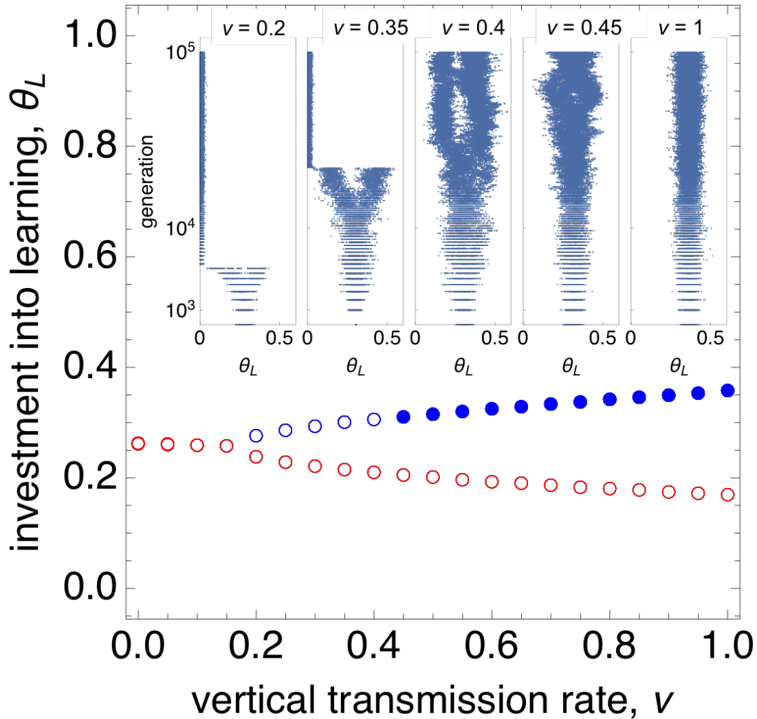
Supplementary Figure 1: Evolutionary branching and vertical transmission. Outset: Interior singular learning strategies of \theta_L according to vertical transmission rate, generated by computing the roots of the selection gradients (eqs. 29 and 32, other parameters: \alpha = 2 , \beta = 12 , \gamma_1 = 0.7 , \gamma_2 = 5 , \lambda = 0.7 ). For each singular value, we computed their convergence stability and local invadability (Appendix B). Red empty circles indicate singular strategies that are convergence unstable and thus represent threshold values above which learning is favored by selection. Blue empty circles are convergence stable but invadable (i.e., potential evolutionary branching points), while blue filled circles are convergence stable and uninvadable (i.e., ESSs). Hence, the analytical model predict that for 0.4 \leq v \leq 1 selection is stabilizing, for 0.2 \leq v \leq 0.4 selection is disruptive, while for v < 0.2 there is no interior convergence stable point. Inset: values of \theta_L for each individual in the population for every 500 generations under individual-based simulations started at the convergence stable singular value, where different panels correspond to different v values (Appendix E). As predicted by the model, we see that when v > 0.4 , the population remains unimodal, when 0.2 \leq v \leq 0.4 , disruptive selection occurs, which results in evolutionary branching whereby the population splits into two morphs. However, when v decreases too much below 0.4, the two morphs are not maintained in the long run and the population converges to zero learning. This is because evolutionary branching causes the population to cross the threshold value of learning, resulting in the collapse of learning.
