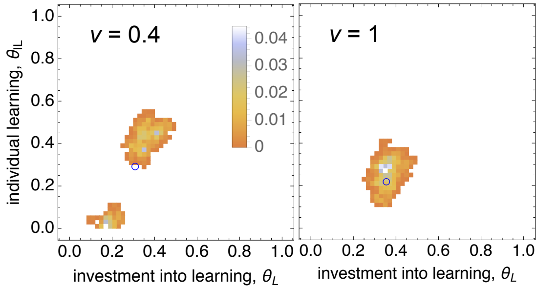
Figure 6: Evolutionary branching and stability. Bivariate distributions of trait values ( \theta_L and \theta_{IL} ), depicted as two-dimensional colour histograms with bins of width 0.02 and in which bin colour gives the frequency of individuals within each bin (see figure legend), obtained under individual-based simulations (frequencies averaged over the last 10^3 generations after 9.9 \times 10^4 generations of evolution, parameters: \alpha = 2 , \beta = 12 , \gamma_1 = 0.7 , \gamma_2 = 5 , \lambda = 0.7 , Appendix E for details). When v = 0.4 , the population is split into two morphs around the interior convergence stable equilibrium ( \theta_L^*, \theta_{IL}^* ) (blue empty circle), but when v = 1 the population is unimodal, centred around the convergence stable equilibrium (blue empty circle).
