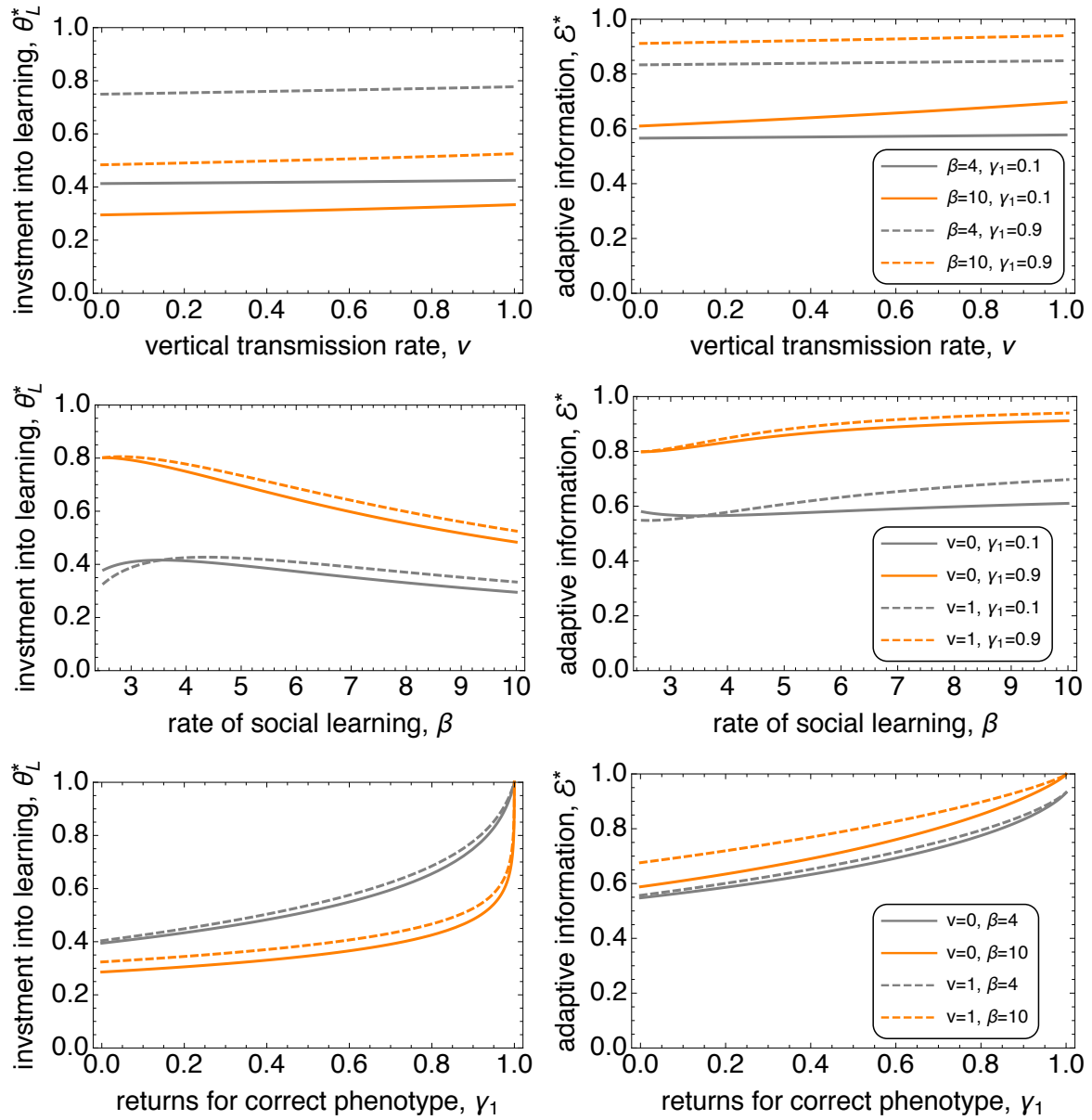
Figure 2: Singular learning strategy \theta_L^* and the corresponding level of adaptive information \mathcal{E}^* it generates (obtained from eqs. (36)-(39)) as a function of the vertical transmission rate v (Top row), the rate of social learning \beta (middle row) and the returns for expressing the correct phenotype \gamma_1 (bottom row). Different lines (gray, orange, full and dashed) stand for different parameter values, whose values are shown in the inset of each row (rate of individual learning is fixed \alpha = 2 everywhere).
