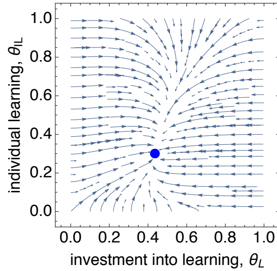
Figure 3: Phase portrait of the co-evolutionary dynamics of \theta_L and \theta_{IL} given by the selection gradients on each corresponding trait (eqs. 29 and 32 using eqs. 34–35 and \lambda = 0 , other parameters: \alpha = 1 , \beta = 8 , and \gamma_1 = 0.5 and v = 0.75 ). The evolutionary dynamics converge to the single interior point shown in blue ( \theta_L^* = 0.436 , \theta_{IL}^* = 0.306 ), which is convergence stable as can be seen from the graph, and which can also be shown to be locally uninvadable (using Appendix B).
