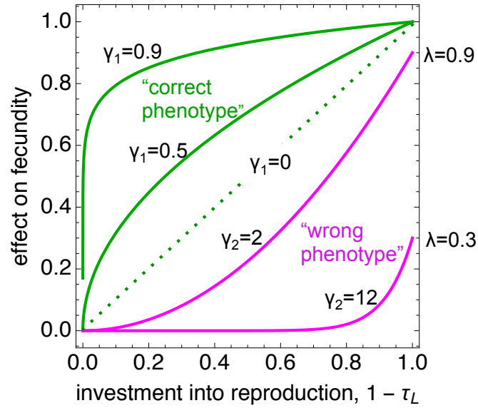
Figure 1: Components of the fecundity function (eq. (35)) as a result of expressing the correct or wrong phenotype. When a mutant expresses the correct phenotype, it obtains rapidly rising returns on investment ( (1 - \tau_L)^{1-\gamma_1} where 0 \leq \gamma_1 < 1 tunes the sharpness of the rise, in green). When a mutant expresses the wrong phenotype, it obtains slowly rising returns on investment ( \lambda(1 - \tau_L)^{\gamma_2} where \gamma_2 > 1 controls how slowly the returns are and 0 \leq \lambda < 1 bounds the returns, in pink). The total effect on fecundity eq. (35) is then given by the average returns, averaged over the probabilities of expressing the correct ( \mathcal{E}(\tau, \theta) ) and wrong ( 1 - \mathcal{E}(\tau, \theta) ) phenotype.
