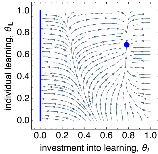
Figure 5: Phase portrait given by the selection gradients on each trait (eqs. 29 and 32 with v = 0 , \alpha = 2 , \beta = 3 , \gamma_1 = 0.9 , \gamma_2 = 3 , \lambda = 0.7 ) and evolutionary convergence equilibria shown in blue (blue line for zero, and filled blue circle for convergence stable interior point), which shows that either \theta_L converges to zero, or both \theta_L and \theta_{IL} converge to an interior equilibrium (\theta_L^*, \theta_{IL}^*) depending on the initial population values. As the graph shows, the co-evolutionary dynamics of \theta_L and \theta_{IL} exhibit bistability and the population must cross a threshold level of learning in order for selection to favor greater investment into learning.
