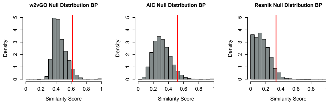
Figure 1: The distribution of similarity scores for many randomly chosen pairs of genes in the BP ontology.
