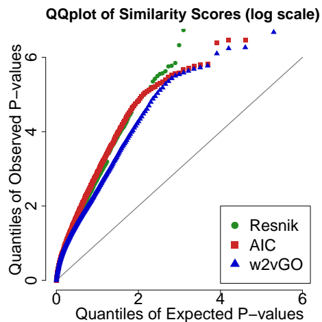
Figure 2: QQ plot of p-values for similarity scores of genes in the same regulatory pathways. BP ontology is used.
