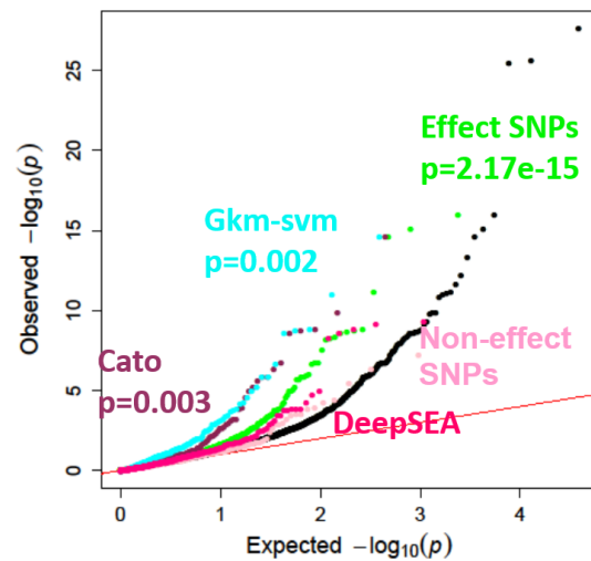
Fig. 3. Validating computational genomic annotations. QQ plot depicting the p -value distributions from testing for ASE using QuASAR, overlapping with computational genomic annotations in LCLs. Effect-SNP scores have a threshold of < -3 or > 3 . CATO Maurano et al. (2015) prediction scores have a threshold of > 0.1 . GKM-svm Lee et al. (2015) gapped kmer sequence-based computational method to predict the effect of regulatory variation has a threshold of < -6 or > 6 . DeepSEA Zhou and Troyanskaya (2015) predicts genomic variant effects at the variant position using deep learning-based algorithmic framework. The functional significance predictions have a threshold of < 0.05 .
