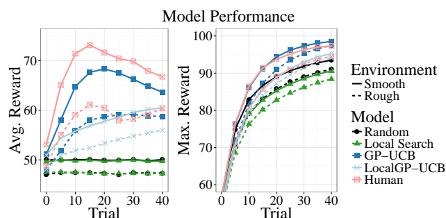
Figure 5: Comparison of simulated model performance over 10,000 replications, where parameters were sampled from the cross-validated MLEs of the subject population. Human results are averaged across payoff conditions and horizon length.
