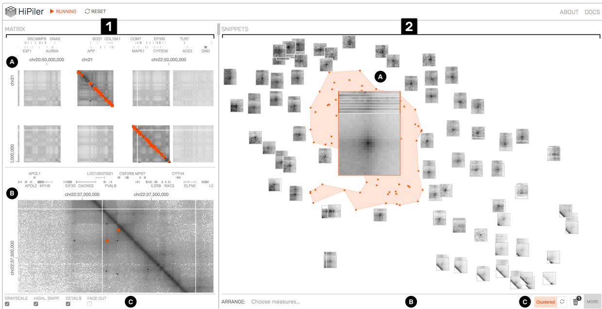
Fig. 1. HiPiler interface: the matrix view (1) with an overview (1A) and detail (1B) matrix. The snippet view (2) presents regions of the matrix as interactive small multiples. In this example, snippets are arranged with t-SNE (2C) and a well-pronounced pile of snippets is highlighted (2A). View menus for operation are located at the bottom (1C and 2B).
