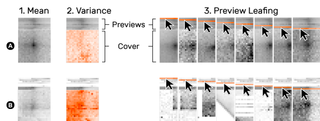
Fig. 12. Snippet aggregation of a more homogeneous (A) and diverse (B) set of snippets. The default cover shows the mean of snippets on a pile (1). The variance cover mode (2) highlights the deviation of snippets. Moving the mouse cursor over a pile’s previews temporarily shows the corresponding snippet or pile (3).
