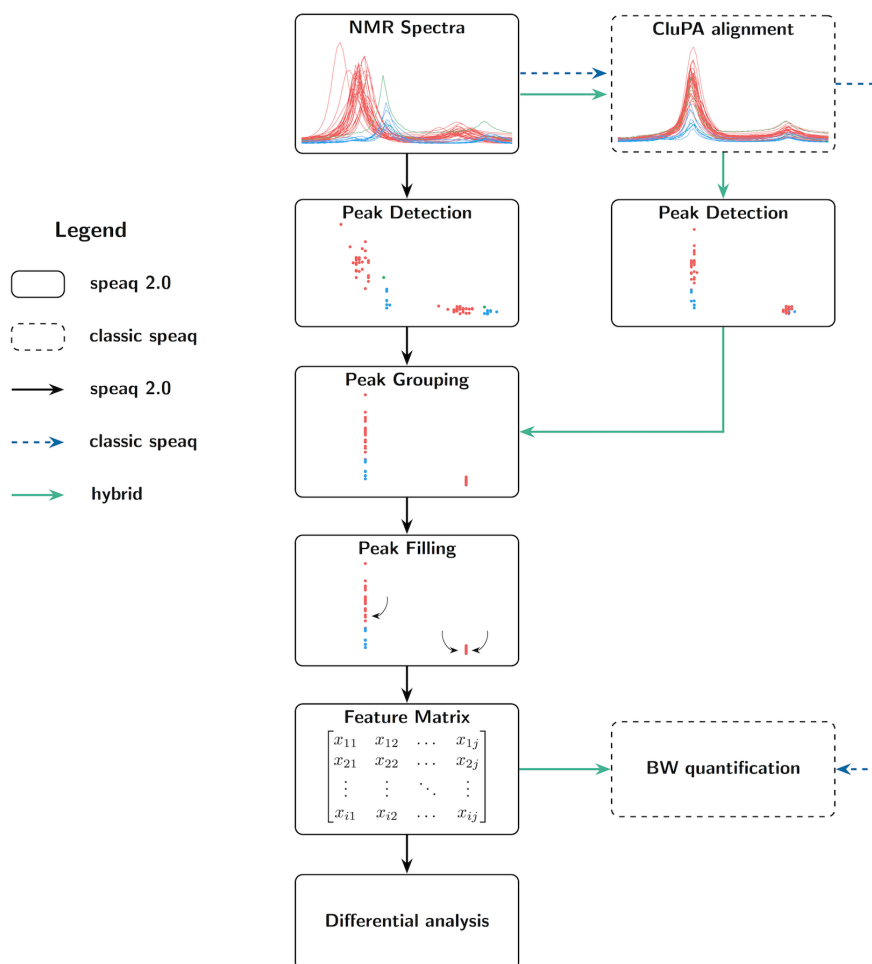
Fig 1. Possible workflows of speaq 2.0. The newly presented methods are standalone (black arrows) or can be used together with the CluPA alignment algorithm [7] (green arrows). It is still possible to perform an analysis based on raw spectra alone, as per the classic speaq analysis. In the new methods raw data is converted to peaks, and every peak is summarized with ppm location and width, intensity and SNR. These peaks are subsequently grouped and optionally peak filled (missed peaks in samples are specifically searched for). The resulting data is converted to a feature matrix that contains intensities for each peak and sample combination. This matrix can then be used in statistical analysis with built-in or external methods.
