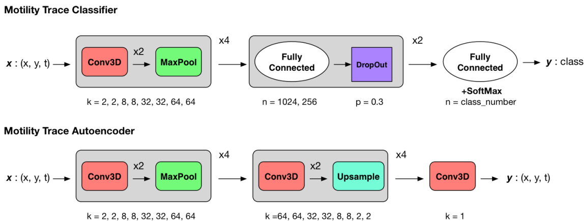
Fig. 2. Motility analysis CNN classification and autoencoder architectures. All convolutional layers are three dimensional and paired with a rectified linear unit activation. Pooling and upsampling layers operate with kernels of size (2, 2, 2) and stride of 2. Zero padding is performed as needed in the autoencoder model to match input size. Here, k is the number of kernels learned by each convolutional layer, n is the number of units in a fully connected layer, and p is the proportion of neurons dropped in a Dropout layer.
