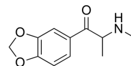
Methylone
