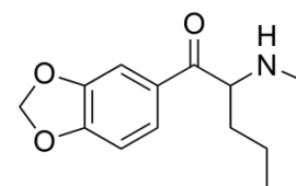
Pentylone
