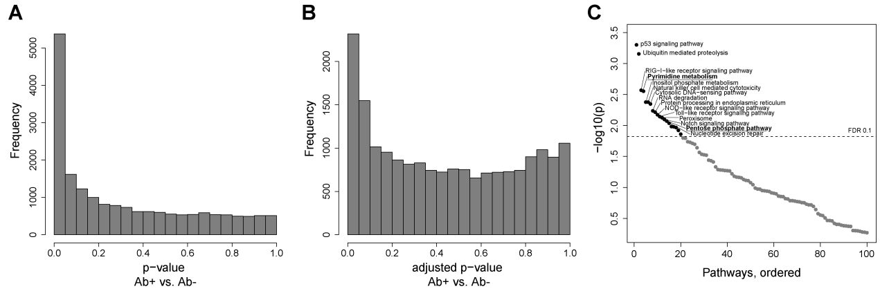
Figure 3: Ab+ analysis. A: Histogram of unadjusted p-values from single gene analysis of islet autoimmunity positive vs. age-matched children who did not develop islet autoimmunity. B: Histogram of p-values after multiple testing, controlling the false discovery rate. C: Sorted -\log_{10}(p) -values of pathway enrichment for islet autoimmunity status. Dashed line indicates the multiple testing threshold at an FDR of 0.1. Abbreviations: Ab+ = Islet autoantibody-positive, Ab- = Islet autoantibody negative.
