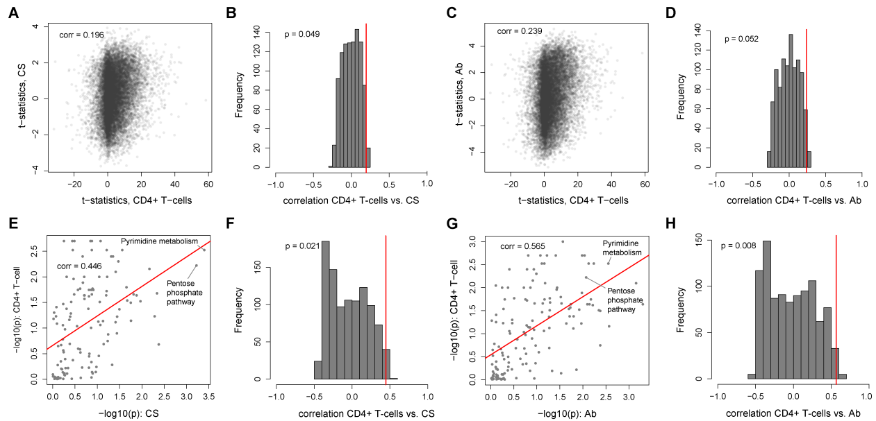
Figure 5: Signatures of immune cell activation- A: Correlation between single gene effects in Cesarean section (CS) compared to the association between naïve and activated CD4+ cells. B: Histogram of correlation of permuted class labels of CD4 T cells and Cesarean section at the single gene level and the “true” correlation effect. C: Correlation between single gene effects in islet autoimmunity status (Ab) compared to the association between naïve and activated CD4+ cells. D: Histogram of correlation of permuted class labels of CD4 T cells and islet autoimmunity status at the single gene level and the “true” effect. E: Correlation between pathway effects in Cesarean section compared to the association between naïve and activated pathways for CD4+ cells. F: Histogram of correlation of permuted class labels of CD4 T cells and Cesarean section at the pathway level and the “true” effect. G: Correlation between pathway effects in islet autoimmunity status compared to the association between naïve and activated pathways for CD4+ cells. H: Histogram of correlation of permuted class labels of CD4 T cells and islet autoimmunity status at the pathway level and the “true” effect.
