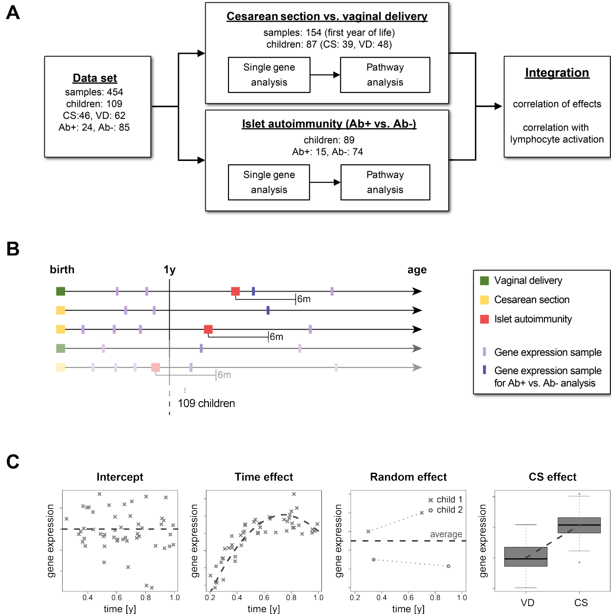
Figure 1: Overview. A: Study workflow: Parallel analyses were performed to detect differential gene expression and pathway enrichment for Cesarean section and islet autoimmunity. The results were then compared in a combined analysis and related to expression patterns of lymphocyte activation. B: Schematic overview of the longitudinal study design for Cesarean section and islet autoimmunity analyses. C: Schematic illustration of the generalized additive mixed effect model (GAMM) to analyze the longitudinal dataset, including intercept, a time effect, a random effect for multiple measurements, and the investigated Cesarean section vs. vaginal delivery effect. Abbreviations: CS = Cesarean section, VD = Vaginal delivery, Ab+ = Islet autoantibody-positive, Ab- = Islet autoantibody-negative.
