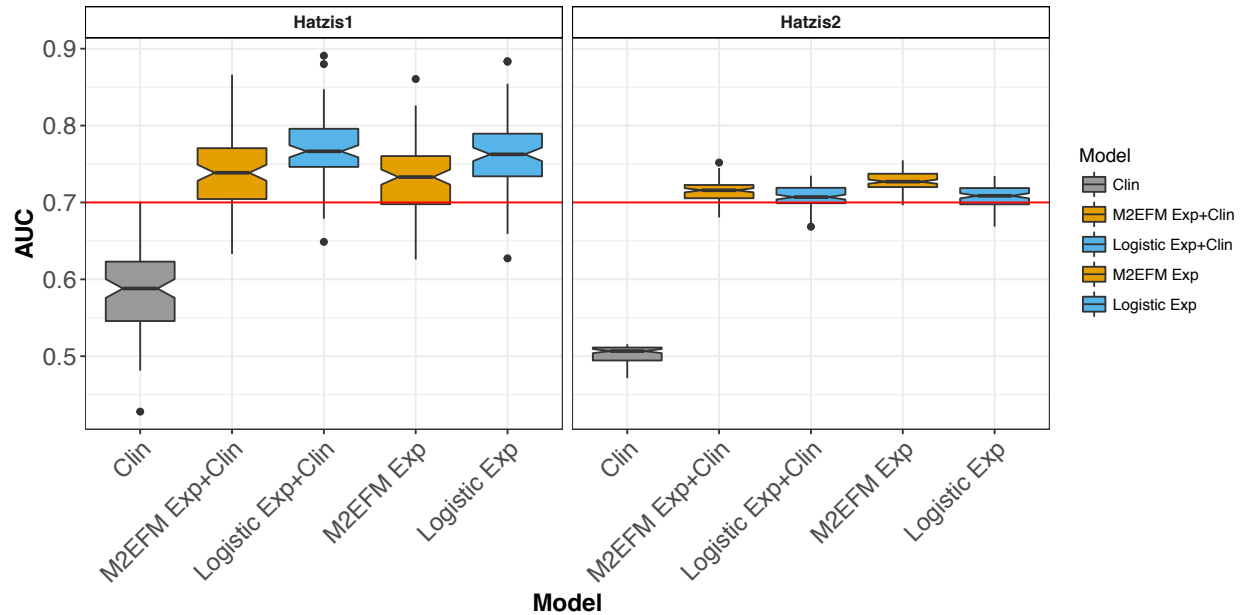
Figure 4: AUC for expression-only pCR models across 100 random splits of Hatzis1 data into training and testing data for the various approaches, which were then validated on Hatzis2. Although Logistic-Ridge models performed better on the internal validation models, M2EFM models performed better on external validation data.
