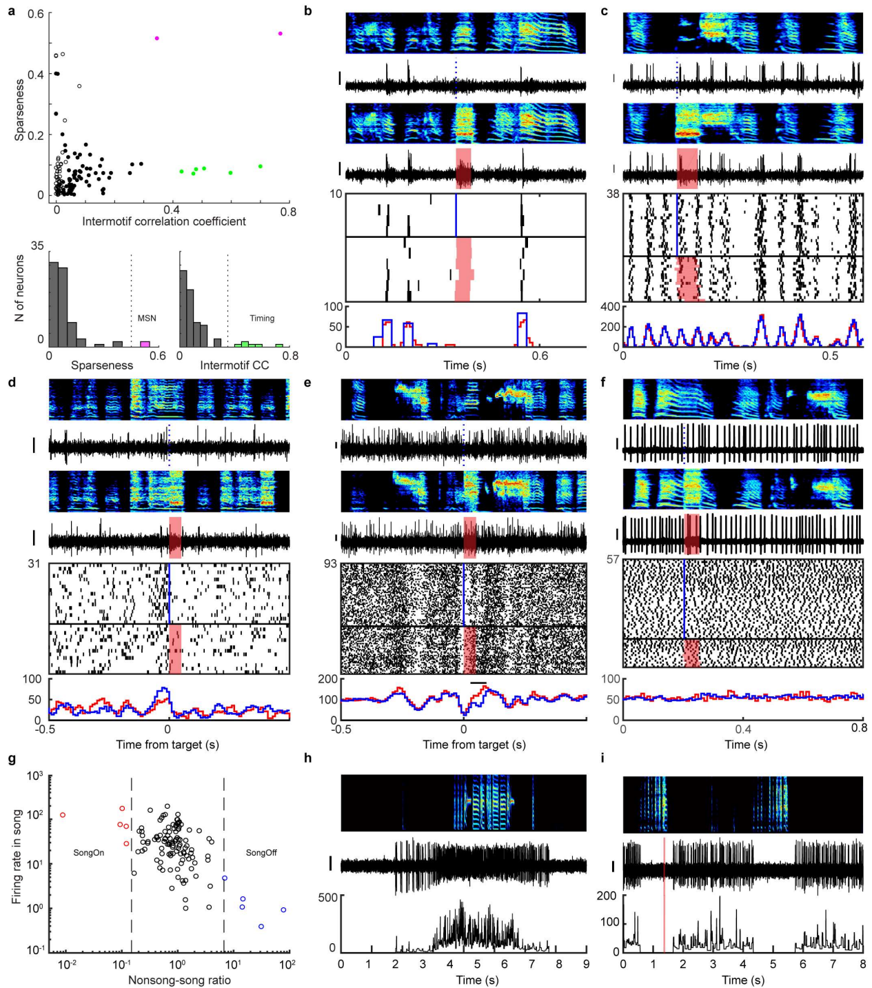
a , Sparseness and intermotif correlation coefficient (ICC) distinguished two classes of time-locked vBG neurons. b , MSN-like vBG neuron with sparse bursts time-locked to song motif. c , vBG neuron with stereotyped high frequency bursts that tile the song motif. d , Pre-target bursting neuron with high firing rate immediately before song target. e , Pre-target pause neuron that was also error-activated. f , vBG neuron unrelated to singing. g , The ratio between mean
