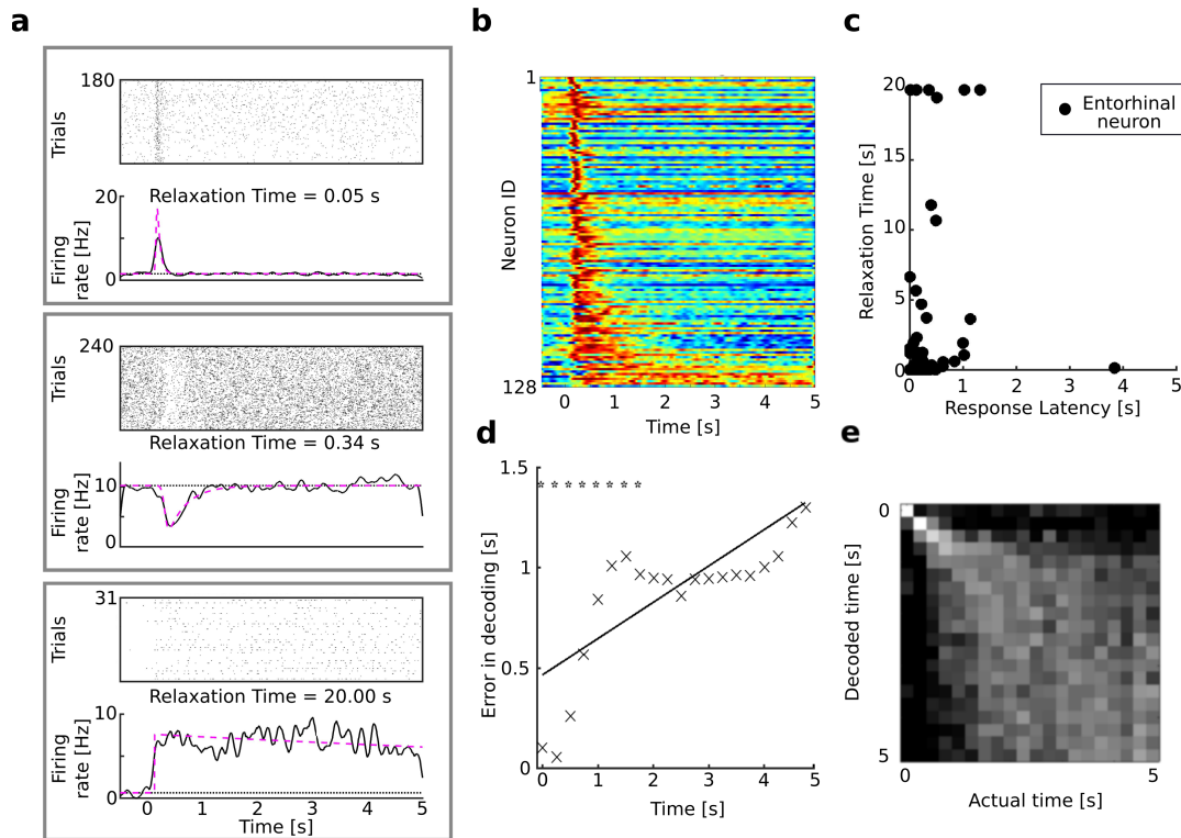
Figure 2. : Temporal context cells in entorhinal cortex respond to the presentation of an image, then relax with a variety of rates, carrying information about time since the image was presented.
