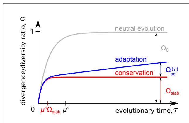
Figure 2: Evolutionary modes and inference of selection for quantitative traits. The figure shows the universal divergence-diversity ratio \Omega , as defined in eq. (2), for a quantitative trait evolving in a single-peak fitness land- or seascape. This ratio is plotted as a function of evolutionary time \tau . Neutral evolution : The function \Omega(\tau) reaches the saturation value \Omega_0 = 1 for large times (grey curve). Conservation : This function has a smaller saturation value \Omega_{\text{stab}} , which is reached faster than for neutral evolution (red curve). Adaptation : There is a linear surplus \Omega_{\text{ad}}(\tau) , which measures the amount of adaptation (blue curve). This behavior can be used to infer selection, as detailed in Box 2.
