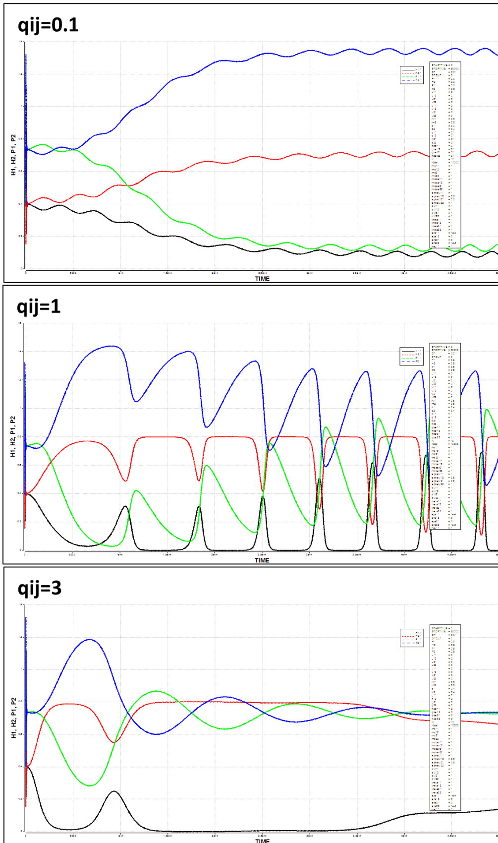
Figure 9. Evolutionary trade-off does not always result to oscillatory behavior. There is a range of parameter value that generates oscillations.
