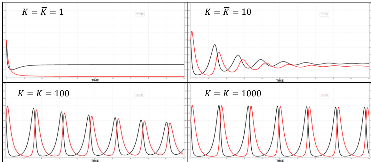
Figure 4. A larger carrying capacity induces oscillation.
