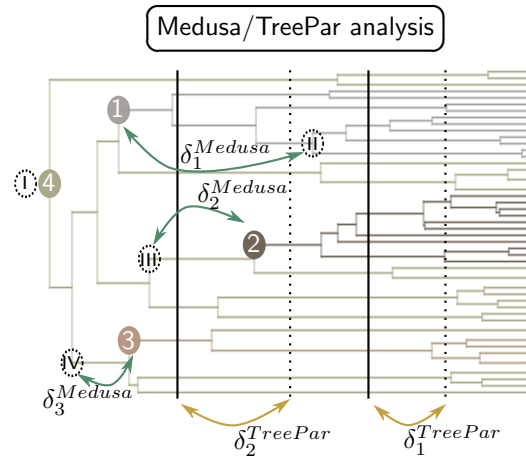
Figure 2 – Example output of the analyzes. We run the Medusa and TreePar analysis, and group the pairs of simulated/estimated events by minimizing the sum of the distance separating the events in each pair ( \sum_i \delta_i^{Medusa} and \sum_i \delta_i^{TreePar} ). Vertical dotted lines: estimated mass extinction events by TreePar, dotted circles with roman letters: estimated diversification rate shift by Medusa, by decreasing significance, other: as in figure 1. The first estimated shift is always at the root of the tree.
