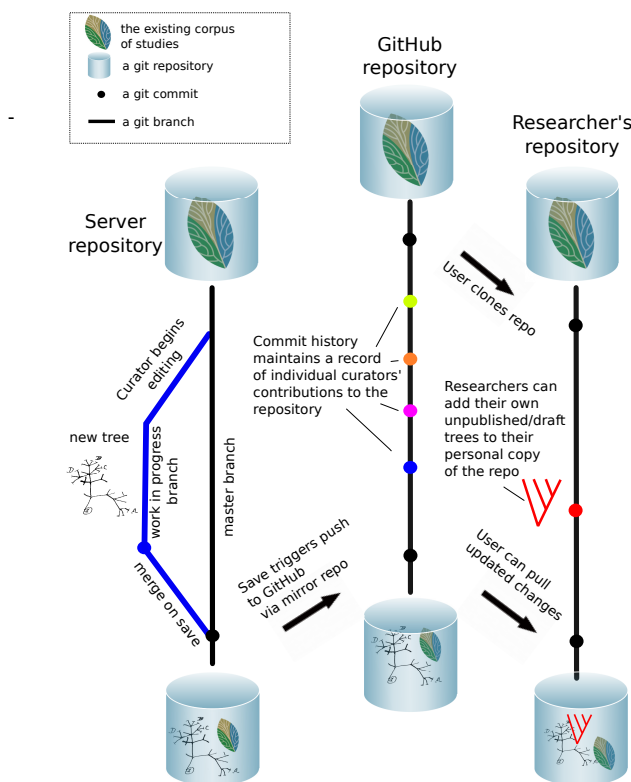
Figure 1: Workflow diagram demonstrating the process triggered by a curator editing a study using the curator app. Upon saving, a work in progress branch is generated on the server repository. If the study edited has not changed on the server, the work in progress branch is merged to master. Merges to master trigger pushes of commits, via the server mirror repository, to the Open Tree of Life GitHub repository. Curation of different studies can proceed independently, and on save each will be merged to master and trigger a push to GitHub. The record of curation changes is readily accessible (here represented with different colors for each curator). Users can easily access changes to the data store, and pull those changes into their own copy of the repository.
