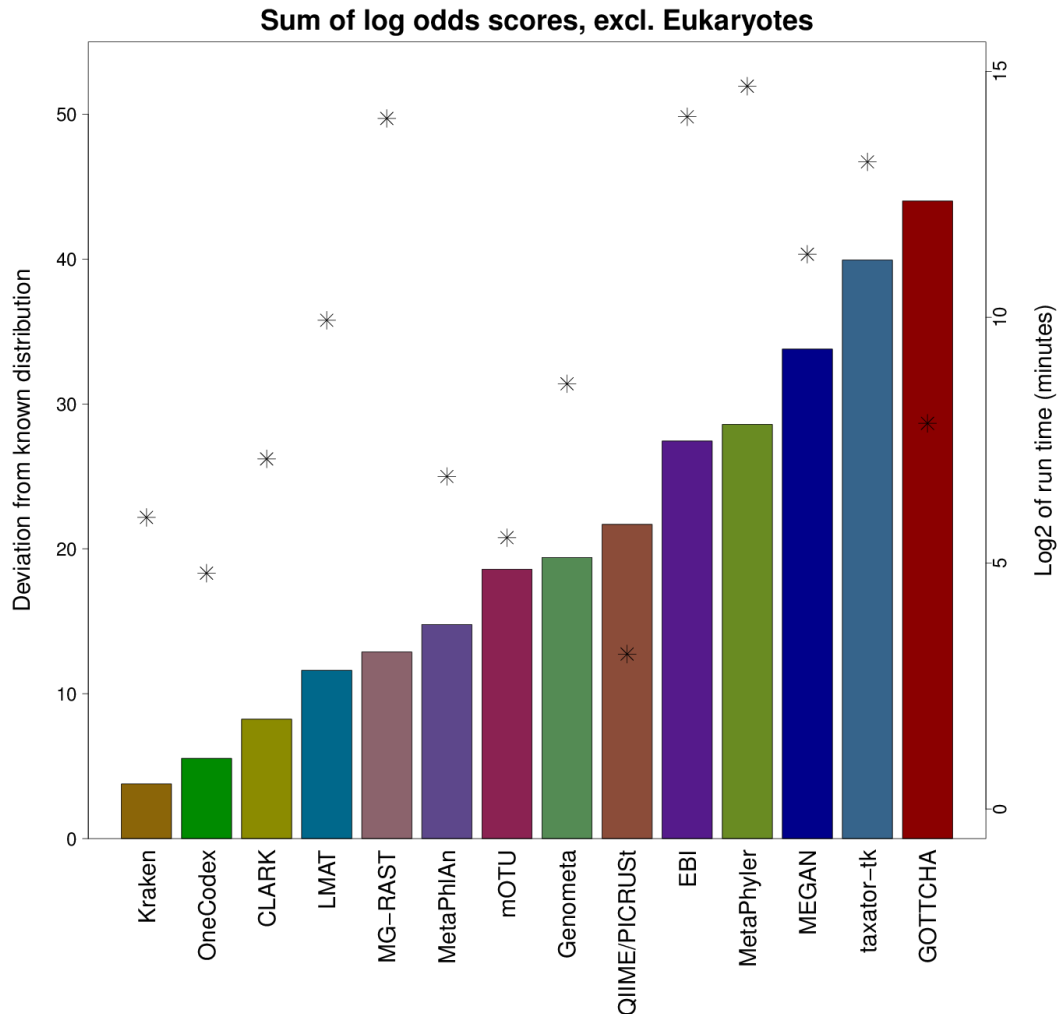
Figure 1: Sum of absolute log odds scores for each tool (bars) and \log_2 of run time in minutes (asterisks, *). Sum of log odds scores indicate the overall performance in terms of deviation from the known proportions. A low sum indicates a high accuracy.
