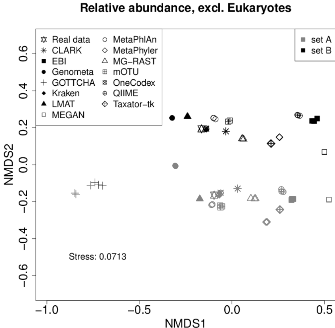
Figure 2: NMDS plot of relative abundances at the phylum level for the known and predicted communities in replicates. Eukaryotes are not included. Metagenomes in set A are gray, and metagenomes in set B are black. The known communities are shown with a star.
