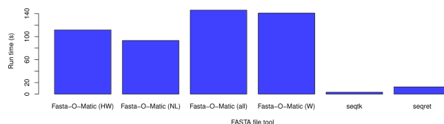
Figure 2: Figure 2 - Run time for various FASTA tools. Tools were run on the Vicugna pacos isolate Carlotta (AHFN-0088) Vicugna pacos -2.0.1 whole genome shotgun sequence NW_005882702.1 with additional unwrapped FASTA sequence record.
