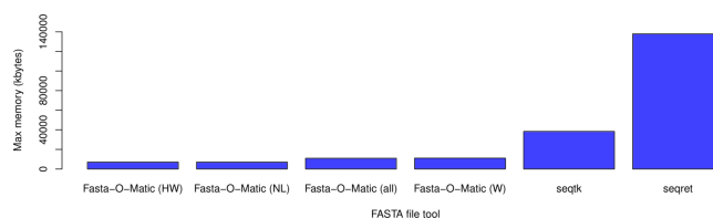
Figure 1: Figure 1 - Max memory used by various FASTA tools. Tools were run on the Vicugna pacos isolate Carlotta (AHFN-0088) Vicugna_pacos -2.0.1 whole genome shotgun sequence NW_005882702.1 with additional un-wrapped FASTA sequence record.
