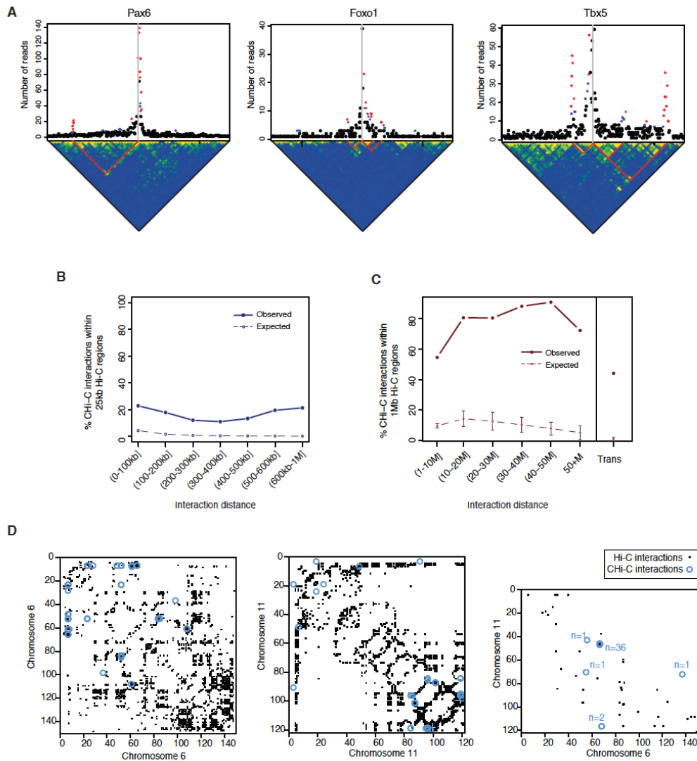
Figure 10. Comparison of interactions detected in CHi-C and Hi-C data. (A) Top panels: Plots showing the read counts from bait-other end pairs within 750kb (upstream and downstream) of 3 baits, containing the Pax6 , Foxo1 and Tbx5 promoters (from left to right). Significant interactions detected by CHiCAGO (score \geq 5 ) are shown in red, and sub-threshold interactions ( 3 \leq \text{score} < 5 ) are shown in blue. Bottom panels: raw Hi-C matrices at 25-kb bin resolution within the corresponding 1.5Mb regions. The bottom corners of the red lines indicate example bin pairs, within which significant interactions were detected in the CHi-C data. (B) Mapping of short-range ( < 1\text{Mb} ) CHi-C interactions within 25-kb interacting bins detected in the Hi-C data. Filled circles show the observed fraction of CHi-C interactions mapping within the Hi-C interacting bins; open circles show the expected fraction estimated by a permutation strategy accounting for genomic structure (see Methods for details). The standard deviations across 100 permutations are not shown as they are smaller than point size. (C) Mapping of long-range ( > 1\text{Mb} ) CHi-C interactions within 1-Mb interacting bins detected in the Hi-C data. Filled circles show the observed fraction of long-range cis - and trans -chromosomal interactions detected in the CHi-C data that map within the Hi-C interacting bins. Open circles show the expected fraction estimated by a permutation strategy accounting for genomic structure (see Methods for details). Error bars show standard deviation across 100 permutations. (D) The overlap of long-range ( > 5\text{Mb} ) interacting fragment pairs detected in CHi-C data (blue circles) and interacting 1Mb bin pairs detected in the Hi-C data (black squares) on chromosomes 6 (left) and 11 (centre), and for trans -interactions between these chromosomes (right). All panels (A)-(D) present mouse pre-capture ES-cell Hi-C data from [4].
