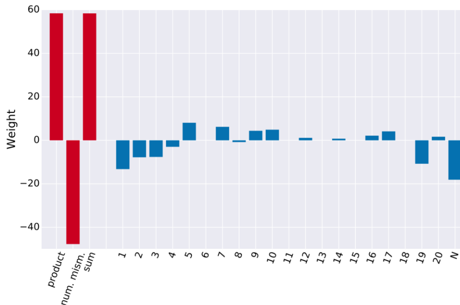
Figure 4. Second-layer guide-target scoring feature importances Weights from second-layer predictive model in Elevation—an L1-regularized regression. This model uses (the log of) the single-mismatch predictions from the first layer as inputs (one for each position in the 20-mer guide and the N position of the PAM, using a 1.0 if no mismatch occurred at that position), shown in blue. The remaining inputs are the product of these non-logged values of these features, as well as their sum, and number of mismatches (and alternate PAM) in the guide, shown in red. The use of the product feature by itself, without the other 23 features would yield the model Elevation-naïve which performs worse. As a consequence, the other features in Elevation can be viewed as a correction of the assumptions in the development of Elevation-naïve, such as independence of mismatches and the regression yielding a true probability.
