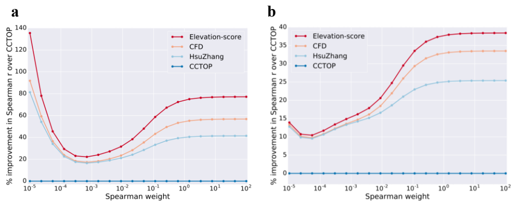
Figure 2. Guide-target pair scoring. Comparison of Elevation-score to other methods, evaluated using a weighted Spearman correlation between predictions and assay measurements. The horizontal axis shows different weights in the weighted Spearman—at the far left the weight is effectively proportional to the rank-normalized GUIDE-Seq counts/cutting frequency, while at the far right the weight is effectively uniform, yielding a traditional Spearman correlation. For ease of visualization, the vertical axis denotes the percent improvement of each model over CCTOP, which by design thus lies constant at zero. (a) CD33 and GUIDE-Seq data were used to train, while Haeussler et al data (after removing the GUIDE-Seq) were used to test. (b) the roles of the GUIDE-Seq and Haeussler data are reversed from a . The final Elevation-score model deployed in our cloud service uses the model trained on GUIDE-Seq data. Note that respectively only 0.12% and 0.51% of count values in GUIDE-Seq and Haeussler are non-zero, making the actual Spearman correlation difficult to interpret. For completeness, however, the right-most points correspond to a correlation of respectively 0.125, 0.111, 0.010 and 0.070 for Elevation, CFD, Hsu-Zhang and CCTOP (left plot) and 0.059, 0.057, 0.053 and 0.043 (right plot). The p-values for each correlation surpassed the floating point error and were reported as p=0.0 in all cases, demonstrating that despite the somewhat low correlations, a tremendous amount of signal is present.
