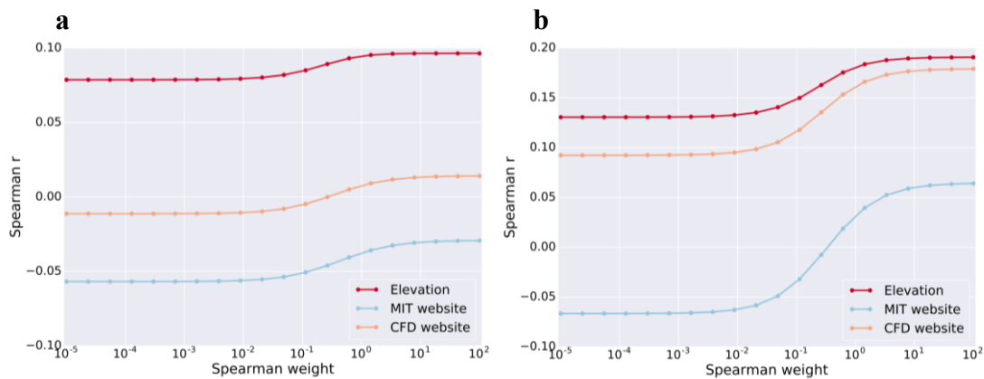
Figure 5. Joint scoring and aggregation on viability screens. Spearman correlation of Elevation to the crispr.mit.edu server. (a) Avana data was used to train and Gecko to test, (b) the reverse of (a) . Note that the MIT website yields correlation in the wrong direction for most settings in both data sets. The final Elevation model deployed in our cloud service uses the model trained on Avana.
