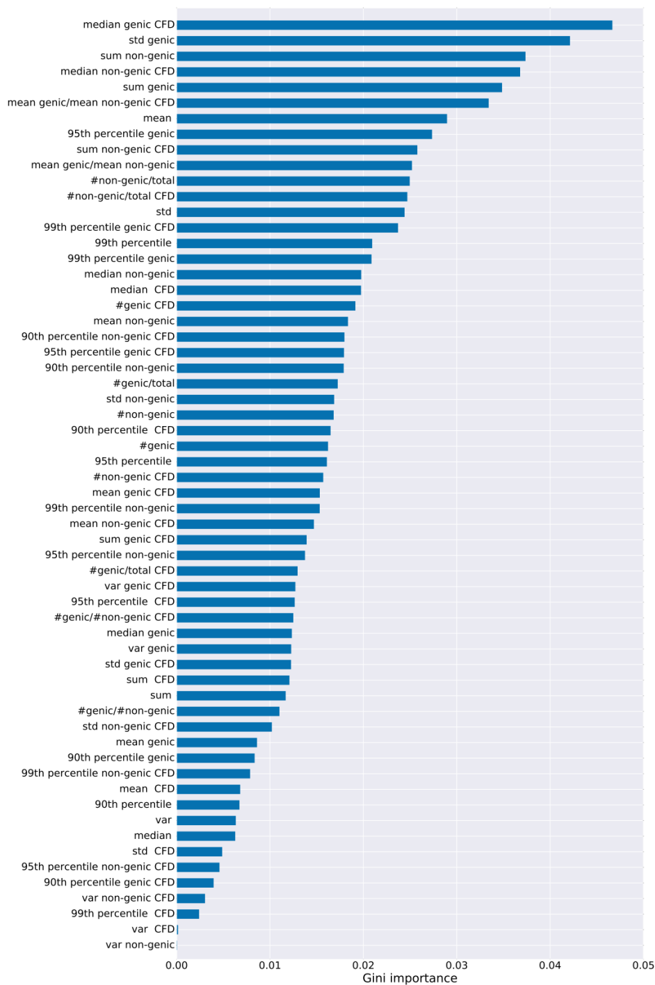
Figure 6. Aggregator feature importances Weights from aggregator model in Elevation which uses Gradient Boosted regression trees. The features were: the mean; median, variance, standard deviation, 99 th , 95 th , 90 th percentiles, and sum of off-target scores. We compute these for each of: all off-targets, only genic off-targets, and only non-genic targets. Additionally, we compute these further features: sum of genic [non-genic] off-targets divided by total number of off-targets; fraction of targets that are genic; fraction that are non-genic; ratio of number of genic to non-genic targets; ratio of average genic to non-genic score. Those with a postfix of “CFD” are from that model, while all others are from Elevation-score. The Gini importance is described in Figure 3.
