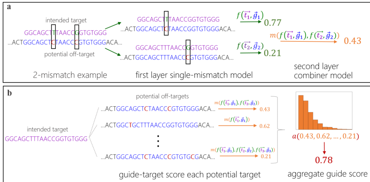
Figure 1. Schematic of Elevation off-target predictive modelling. (a) An example of how to score a guide-target pair with two mismatches. First the guide-target pair is broken down into two single-mismatch pseudo-pairs, each of which is scored with the first layer model. Then these scores are combined with the second-layer model, yielding a single guide-target score. (b) An example how to aggregate the set of guide-target scores for a single guide into one summary off-target score for a guide. The aggregator model computes statistics of the input distribution of guide-target scores as features for the model.
