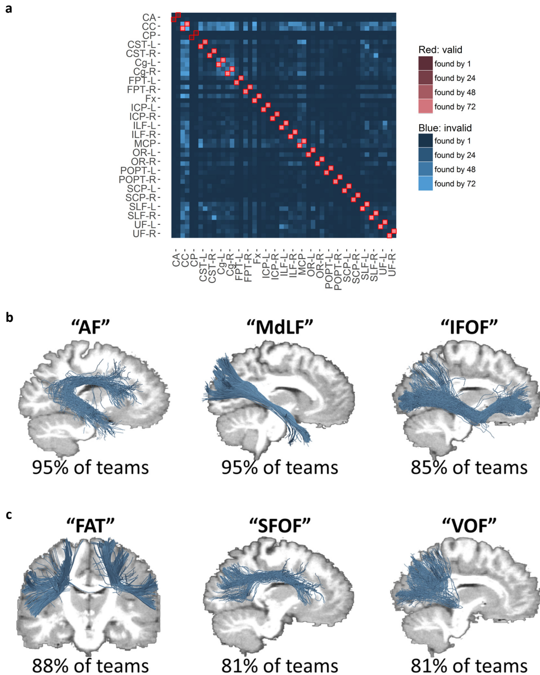
Figure 4. Overview of valid (red) and invalid (blue) bundles. Clusters of invalid streamlines exhibit similarities to previously reported, yet unconfirmed bundles from the literature. (a) Each entry in the connectivity matrix indicates the number of submissions that have identified the respective bundle. The two rows/columns per bundle represent the head-endpoint and tail-endpoint regions of a bundle. (b, c) The shown invalid bundles have been consistently identified by more than 80% of the teams, but do not exist in the ground truth. As discussed in the main text, some of these bundles exhibit a high similarity to bundles that are known to exist, as shown in (b), including the arcuate fasciculus (AF) and bundles traversing the temporal stem such as the middle longitudinal fasciculus (MdlF) and the inferior-frontal occipital fasciculus (IFOF). Other bundles – shown in (c) – are not known to exist and are debated in literature. These include the frontal aslant tract (FAT), the superior fronto-occipital fasciculus (SFOF) and the vertical occipital fasciculus (VOF).
