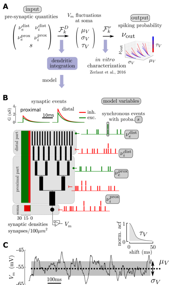
Figure 1. A theoretical framework for single cell computation in the fluctuation-driven regime: cellular model and two-step approach for the input-output function. (A) Theoretical paradigm: to get the input-output function of a single cell, we split the relation from presynaptic quantities (the input) to the spiking probability (the output) into two steps. 1) passive dendritic integration shapes the membrane potential at the soma and 2) how those fluctuations are translated into spikes is captured by a firing response function determined in vitro . (B) Theoretical model for dendritic integration. A single cell is made of a lumped impedance somatic compartment and a dendritic tree. The dendritic tree is composed of B branches (here B=5 ), the branching is symmetric and follow Rall's 3/2 rule for the branch diameters. Synapses are then spread all over the membrane according to physiological synaptic densities. We define 3 domains: a somatic and proximal domain as well as a distal domain, excitatory and inhibitory synaptic input can vary independently in those domains. An additional variable: synaptic synchrony controls the degree of coincident synaptic inputs. (C) A given presynaptic stimulation (here v_e^p = v_e^d = 0.2 \text{ Hz} , v_i^p = v_i^d = 1.2 \text{ Hz} and s = 0.05 ) creates membrane potential fluctuations at the soma characterized by their mean \mu_V , their amplitude \sigma_V and their autocorrelation time \tau_V .
