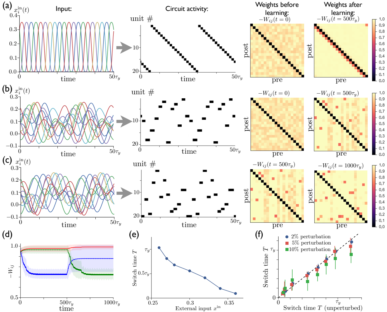
Figure 3: Repeated external input can tutor striatum to produce sparse activity sequences. (a) 20 cycles of a regular sequence of pulse-like inputs (only 10 inputs are shown for clarity; 25\tau_y = 1 cycle) ( left ) leads to a sequential activity pattern ( center ) and, via anti-Hebbian plasticity, converts a random connectivity matrix (at t = 0 ) to a structured matrix (at t = 500\tau_y ) ( right ). (b) Starting with random connectivity between units (at t = 0 ), each unit is driven with a distinct time-varying input consisting of a random superposition of sine waves (two cycles of which are shown for 10 inputs) which produces a repeating activity sequence. Anti-Hebbian learning results in a structured matrix after 20 cycles (at t = 500\tau_y ). (c) 20 cycles with a new input elicits a different activity pattern and overwrites the prior connectivity to a new structured matrix (at t = 1000\tau_y ). (d) The evolution of the synaptic weights during the learning in ‘b’ and ‘c’. The blue, green, and red lines show the average weights of synapses involved in the first pattern, the second pattern, and neither pattern, respectively. (The weights shown in blue are not all repotentialiated in the second training period due to the fact that some of these synapses are from units that are not active in the second sequence. For these weights \bar{x}_j \approx 0 in Equation 2, and thus they do not learn.) (e) The average time for switching from one unit to the next as a function of the constant external input after learning. (f) The switch times are robust to random perturbations of the weights. Starting with the final weights in ‘c’, each weight is perturbed by \Delta W_{ij} = p\xi_{ij}(W_{ij}) , where \xi_{ij} \sim \mathcal{N}(0, 1) is a normal random variable, and p = 0.02, 0.05 , or 0.10 . The perturbed switch times (slightly offset for visibility) are averaged over active units and realizations of the perturbation. Learning-related parameters are \tau_w = 3\tau , \alpha_1 = 0.05/\tau , and \alpha_2 = 0.02/\tau .
