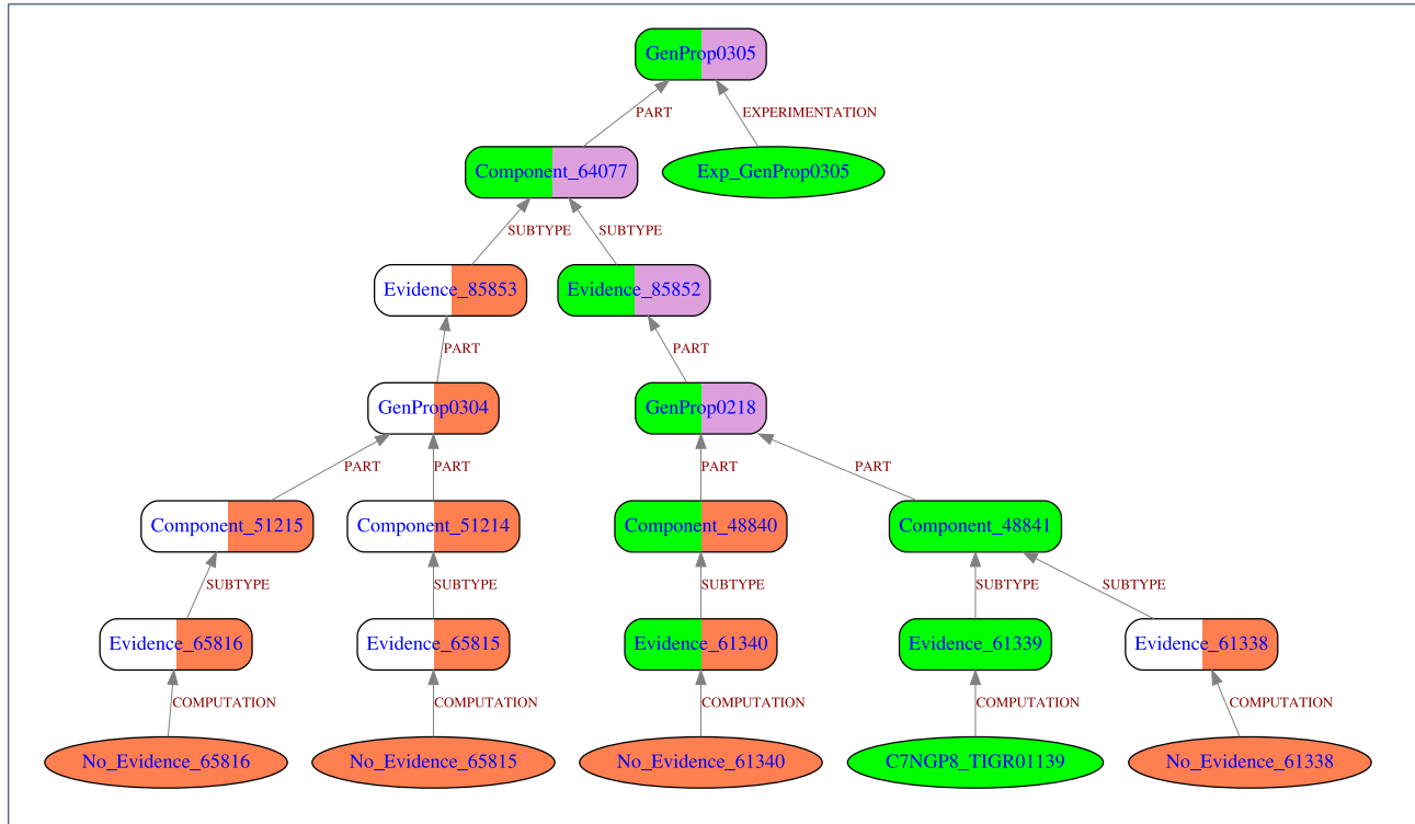
Figure 3 GROOLS results for cysteine biosynthesis in Kytococcus sedentarius .
