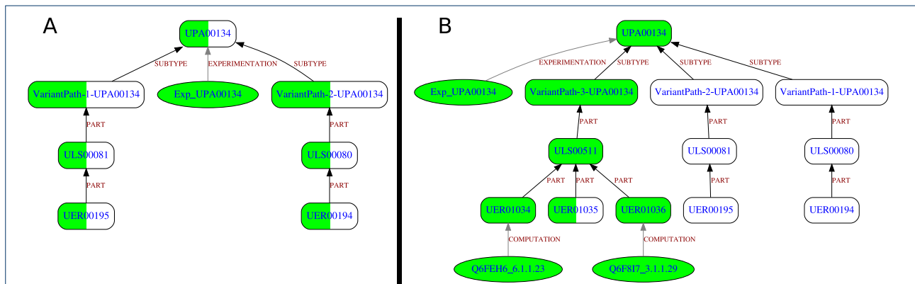
Figure 4 GROOLS results for asparagine biosynthesis in Acinetobacter baylyi .
