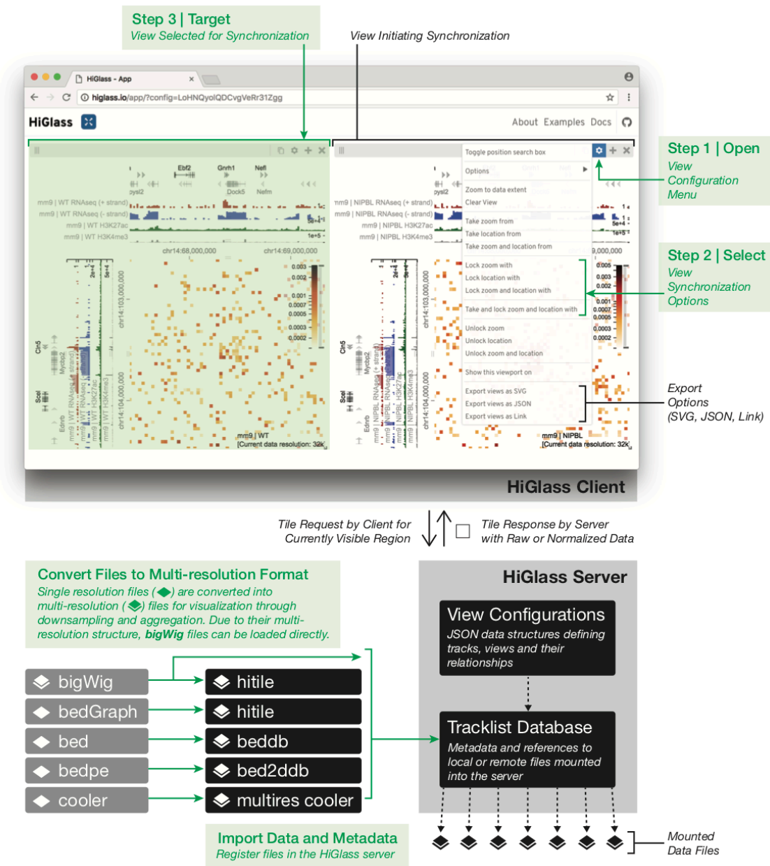
Figure 6 | A schematic of the data flow and user interface of HiGlass. Starting from the bottom-left, single resolution formats used for genomics data are converted to their multi-resolution counterparts. Files in the bigWig format, which is a native multi-resolution format, are directly converted to the hitile format compatible with HiGlass. The multi-resolution files are then loaded into the HiGlass server using a command line tool. The HiGlass client (top half) communicates with the server by issuing ‘tile requests’ for the data that is currently visible in the user’s browser. The server responds with raw data which the client renders into vertical, horizontal and 2D tracks. Within the client, users can zoom and pan around the data or select views with which to synchronize the location, zoom level or both. View synchronization is initiated from one view and tied to another.
