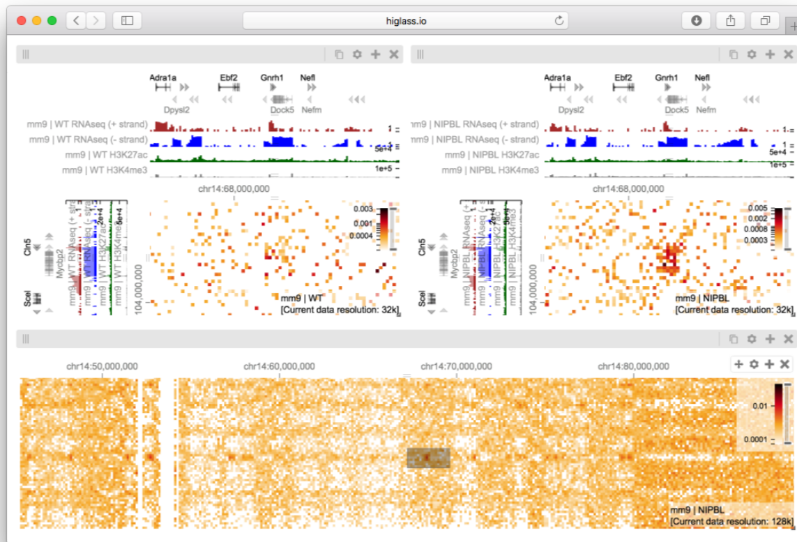
Figure 3 | A view composition containing two views linked by location and zoom (top) and an independent (unlinked) zoomed out overview (bottom) (Supp. Fig. 3). The two views on top show data from chromosome 14 (mm9) in the wild type and \Delta Nipbl conditions, respectively. The bottom view shows data from the mutant condition as well as a projection of the viewport visible in the top views. The patch visible in the \Delta Nipbl condition (top left) is notably absent from the control (right). The gene annotations, RNAseq, H3K27me and H3K4me3 tracks show the presence and transcription of the Dock5 and Mycbp2 genes on the - strand as well as the presence and transcription of the Grnh1 and Cln5 genes on the + strand. An interactive version of this figure is available at http://higlass.io/app/?config=Q5LdNchQRLSZ_0yKsTEoiw .
