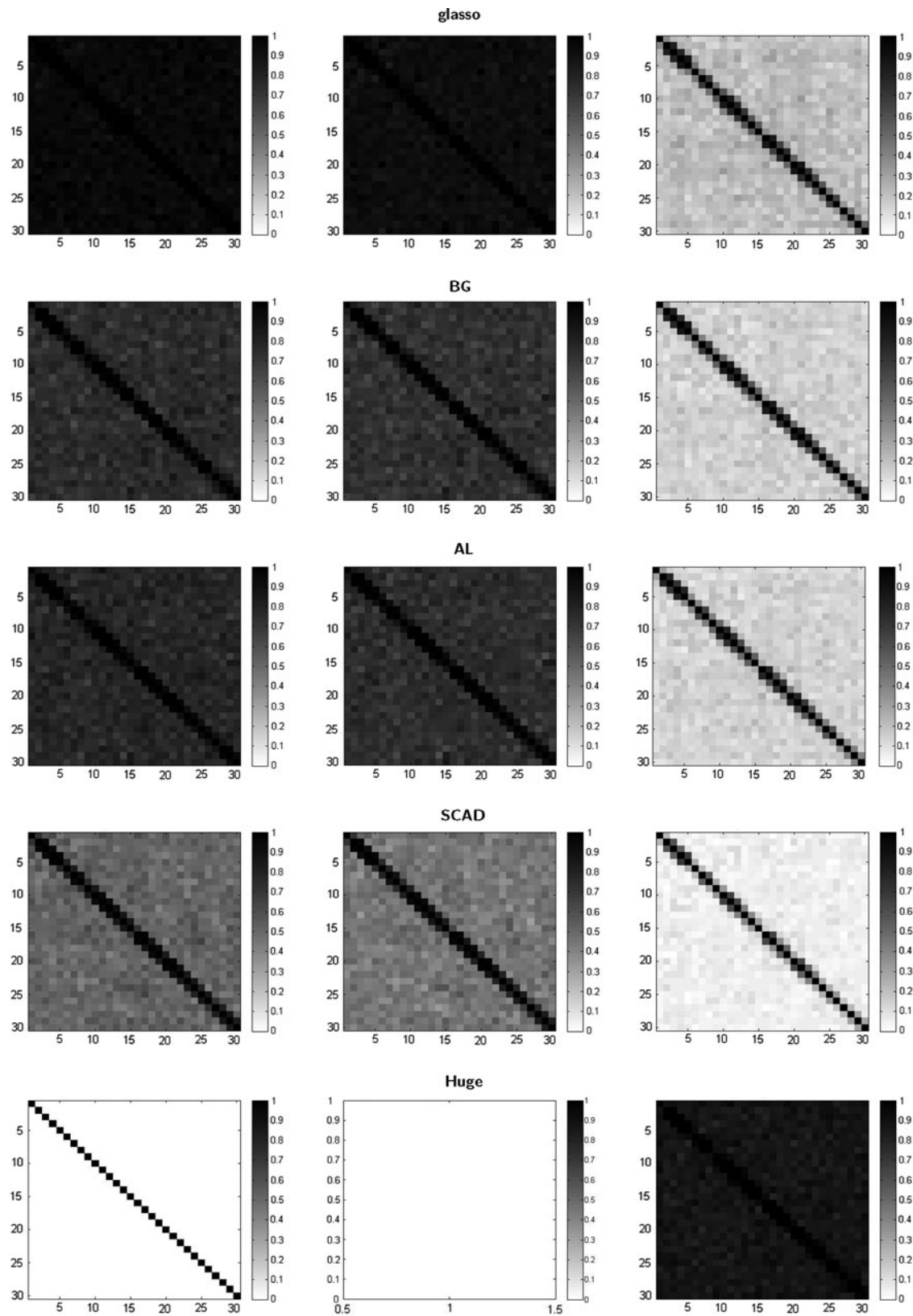
FIG. 6. The ASP plots for the tridiagonal matrix with a = 1.7 for the MVN data with AR1 structure ( p = 30 ) data. The left, middle, and right columns represent the selection criteria AIC, BIC, and CV for estimating methods glasso, BG, AL, and SCAD, and ebic, ric, and stars for Huge, respectively.
