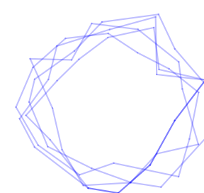
5 reads
