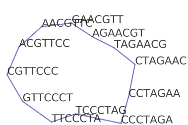
1 reads
