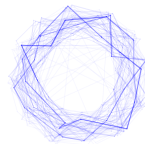
100 reads
