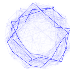
1000 reads
