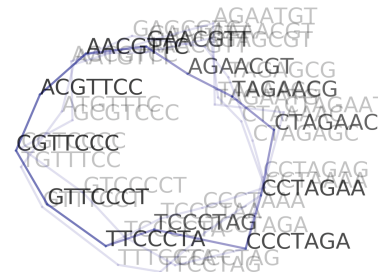
5 reads
