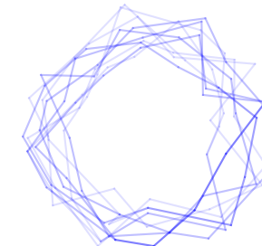
10 reads
