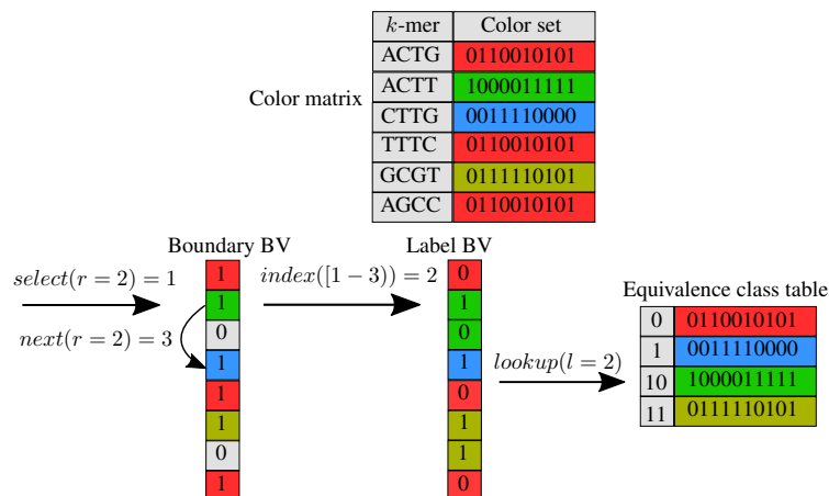
■ Figure 1 The representation of color information in Rainbowfish. The “Color Matrix” at the top represents 6 distinct 4-mers, each assigned a color set. 3 of these 4-mers (ACTG, TTTC, AGCC) have the same color class, labeled 0, and the other 3 (CTTG, ACTT, and GCGT) each have color classes labeled 1, 10, and 11 respectively. To retrieve the color set for a k -mer, we first perform select on the boundary bit vector (BBV) using rank r of the corresponding edge ( k -mer). This returns the label’s starting position, i . We then look for the next set bit BBV to find the label’s ending position, j . Then, we fetch the label at indices i to j in label bit vector (LBV). Finally, we lookup the label l in the equivalence class table (ECT) and return the color class corresponding to the label.
