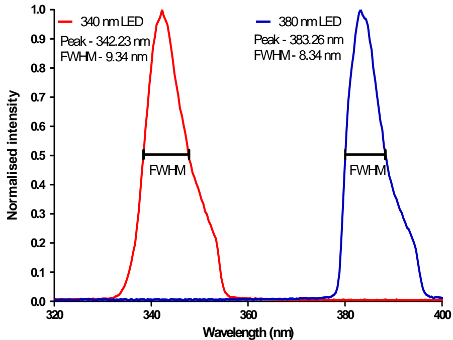
Figure 1; Output spectra of 340/380 nm LEDs obtained at a drive current of 1.52 \pm 0.16 A
