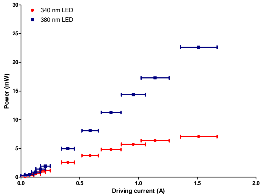
Figure 2; Optical powers measured at the specimen plane of an Olympus BX50 microscope under a 20X water dipping lens at different LED drive currents.
