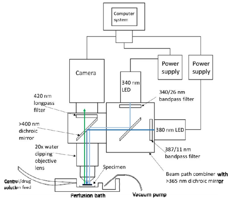
Figure 3; Schematic diagram of experimental imaging setup showing the location of the specimen in relation to the objective lens and where the perfused solution flows over the specimen and gets removed from the bath. The light paths of the 340/380 nm LEDs are also shown to converge through the use of 365 nm dichroic mirror and then illuminate the specimen in the perfusion bath sequentially. The emitted Fura-2 AM fluorescence propagates upwards through the objective lens, >400 nm dichroic mirror (Olympus) and 420 nm longpass filter (Olympus) to the camera. The camera and power supplies for both LEDs are connected to a computer system for TTL triggering and recording fluorescent signals.
