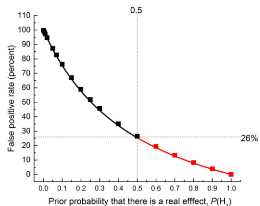
Figure 5, The false positive rate plotted against the prior probability for a test that comes out with a P value just below 0.05. The points for prior probabilities greater than 0.5 are red because it is essentially never legitimate to assume a prior bigger than 0.5.
