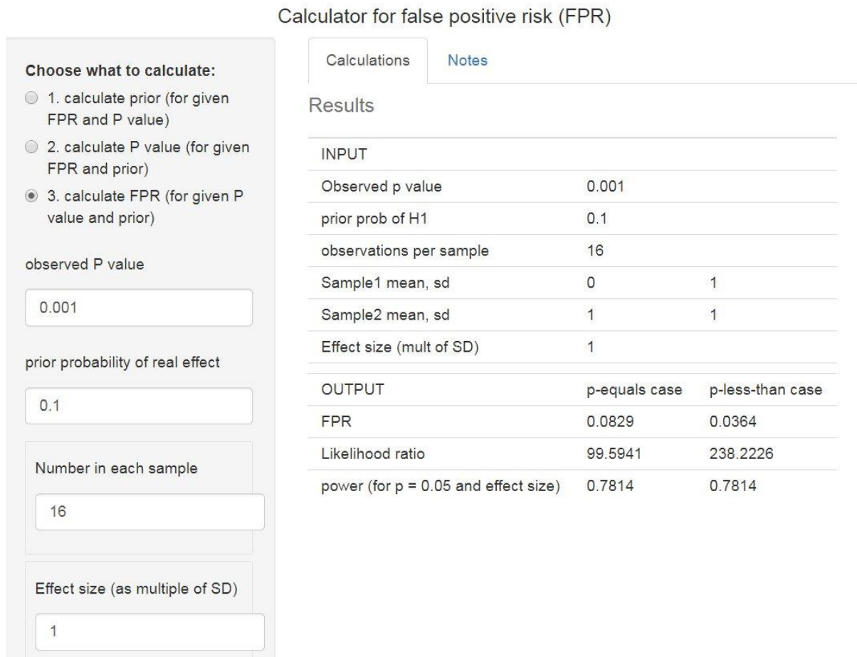
Figure 4. Web calculator [42] for the case where we observe a P value of 0.001 and the prior probability of a real effect is 0.1
