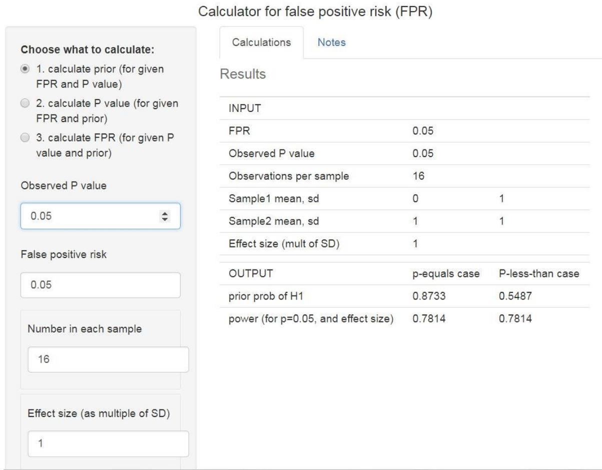
Figure 6. Web calculator: calculation of the prior probability than would be needed to achieve a false positive risk of 5% when we observe P = 0.05 .
