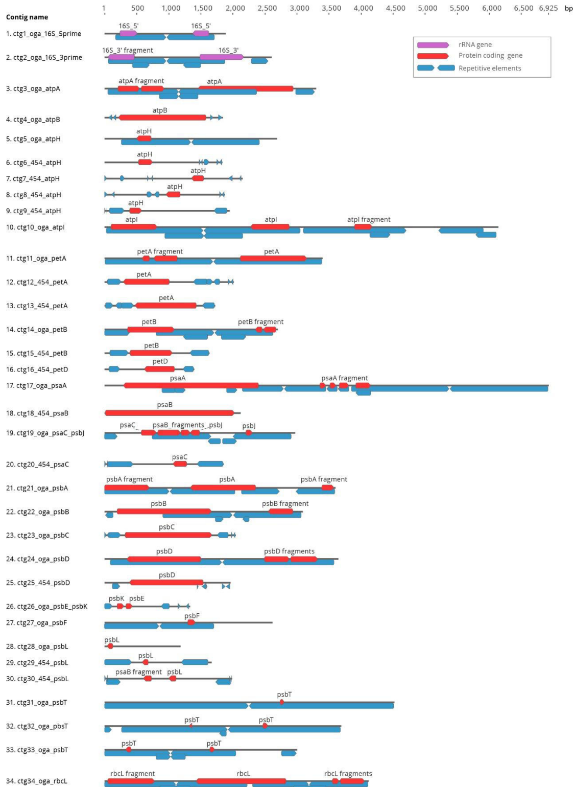
Figure 4 | Schematic representation of Boodlea chloroplast genome. Purple arrows indicate rRNA genes, red arrows indicate CDSs of protein-coding genes, and blue arrows indicate repetitive elements. For each contig, repetitive elements with similar length indicate similar sequences. Oga: contig obtained by orthology-guided assembly. 454: chloroplast 454 contig.
