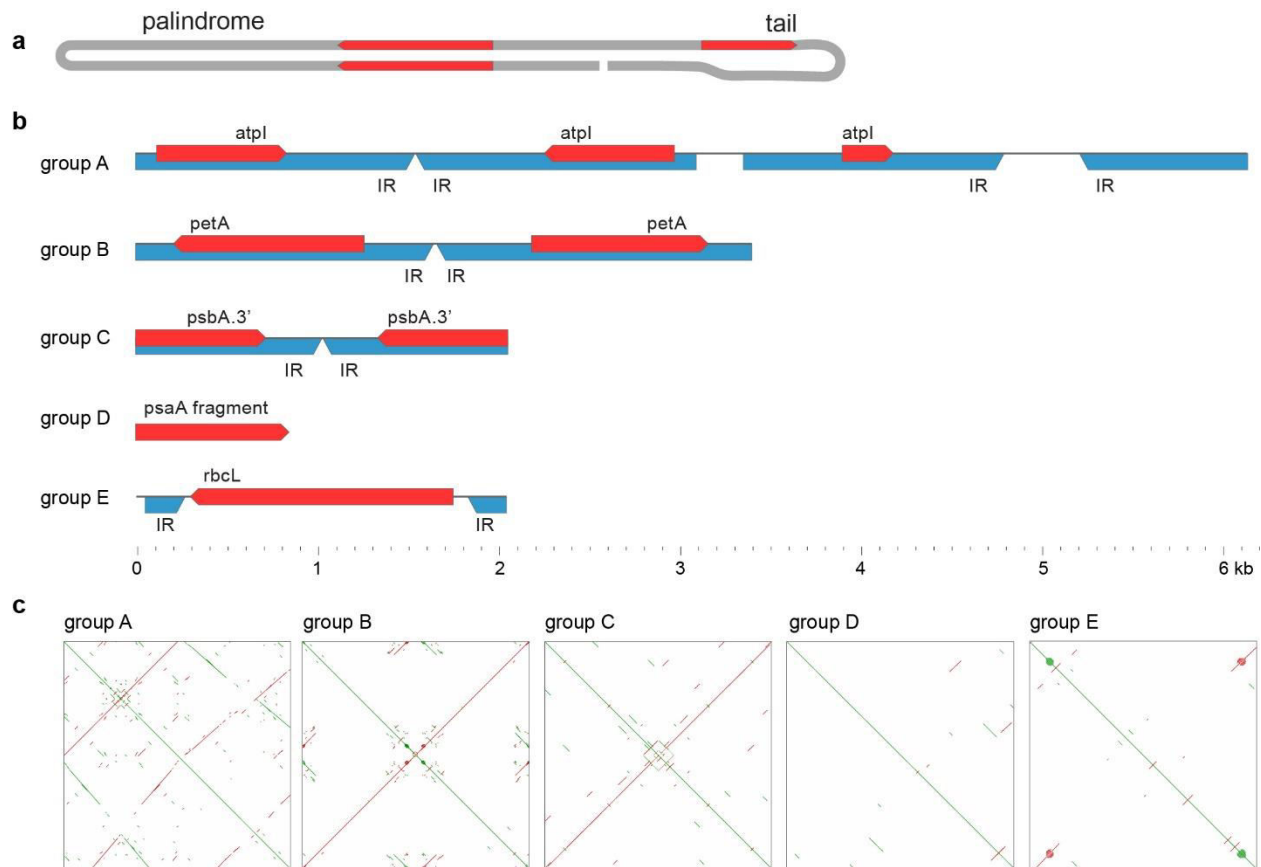
Figure 2 | Schematic representation of assembled Boodlea chloroplast DNA contigs. a. Schematic representation of one of the predicted native conformation of chloroplast hairpins plasmids (with a near-perfect palindromic region and a less conserved tail). Red arrows represent CDSs. b. Schematic representation of the assembled Boodlea chloroplast DNA contigs; red arrows represent CDSs, blue arrows represent major inverted repeats; scale bar at the bottom indicates length of the contigs/reads. Group A: The first half of the read is a perfect palindrome, containing the two inverted CDSs; the second half of the read (tail) is less conserved, but similar to the first half of the read. Group B: Palindromic sequences with full-length CDSs in opposite orientations, resembling the first half of group A read. Group C: palindromic sequences with fragments of CDS. Group D: short reads with fragments of CDSs that lack extensive repetitive elements. Group E: Full-length CDSs delimited by inverted repeats. Similar to group E contigs and reads, the remaining 113 chloroplast 454 contigs lacking full-length CDSs are delimited by inverted repeats. c. Dotplots of the five groups, showing the abundance of repetitive elements. Each dotplot was generated by aligning the contig/read with itself. Green lines indicate similar sequences; red lines indicate sequences similar to the respective reverse complements.
