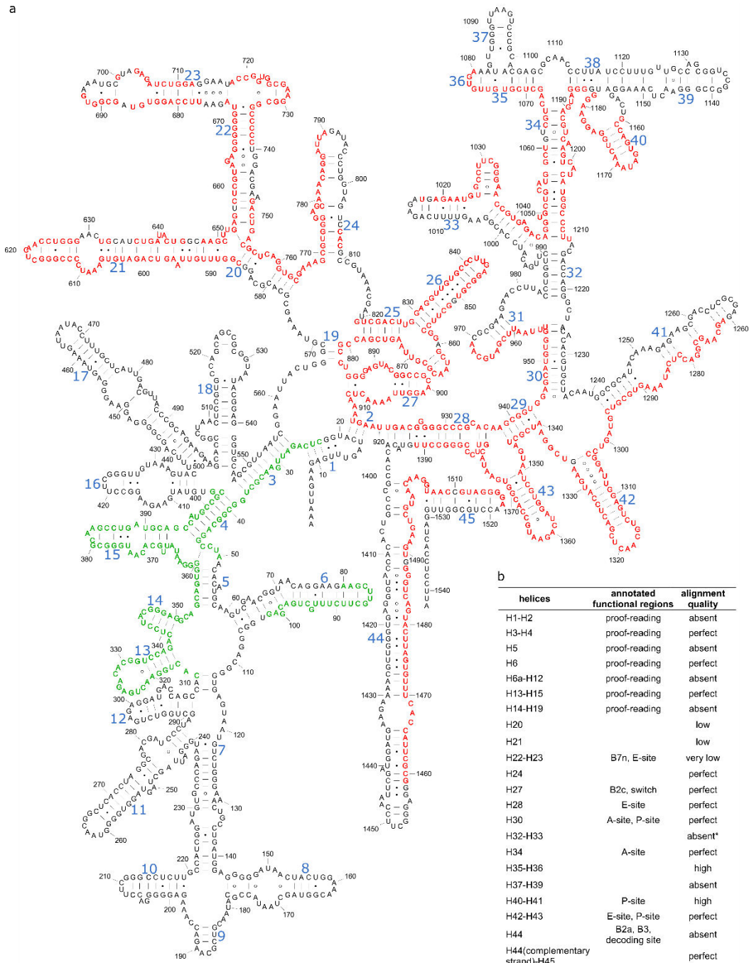
Figure 5 | Boodlea chloroplast 16S rRNA secondary structure. a. Boodlea chloroplast 16S rRNA secondary structure was compared with the E. coli 16S rRNA model [RF00177]. Residues shown in green and red on the E. coli model represent the 5' and 3' 16S rRNA regions coded by the two Boodlea 16S rRNA hairpin plasmids. Residues in black are absent in Boodlea 16S rRNA. Blue numbers indicate secondary structure helices in the 16S rRNA model 102 . b. Comparison between Boodlea and E. coli 16S rRNA annotated functional regions. Quality of the alignment was assessed based on the predicted posterior probability (in percentage) of each aligned region: very low < 25%; low between 25-50%; high between 50-95%; and perfect > 95%.
