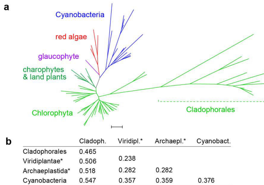
Figure 7 | Phylogeny of Archaeplastida and Cyanobacteria based on 19 chloroplast genes, and corresponding distance matrix illustrating the large sequence divergence of Cladophorales chloroplast genes. a. Maximum likelihood phylogenetic tree inferred from a concatenated amino acid alignment of 19 chloroplast genes. The phylogeny with taxon names and bootstrap support values is shown in Supplementary Fig. 4. The scale represent 0,3 substitution per amino acid position. b. Maximum pairwise amino acid sequence distances of the chloroplast genes within and between clades (* excluded Cladophorales).
