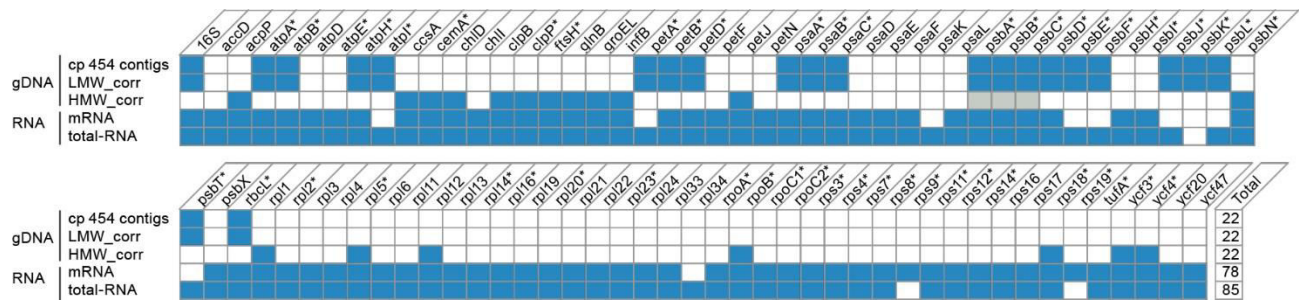
Figure 3 | Boodlea genes having orthologs in the chloroplast of other Archaeplastida and their distribution over the sequenced DNA/RNA. gDNA (genomic DNA): chloroplast (cp) 454 contigs, HMW and LMW corrected reads; RNA: mRNA and total-RNA assemblies. Asterisks (*) indicate "core" chloroplast genes, i.e. protein-coding genes conserved between chloroplast genomes of Chlorophyta (see Methods). The following 9 "core" chloroplast genes were not found in any of the Boodlea libraries sequenced: atpF , petG , petL , psaJ , psbM , psbZ , rpl36 , rps2 and ycf1 . Grey cells are putative carry-over contaminants: LMW DNA reads contaminants as suggested by the ratios of HMW to LMW DNA reads and mRNA to total-RNA reads (Supplementary Fig. 2).
