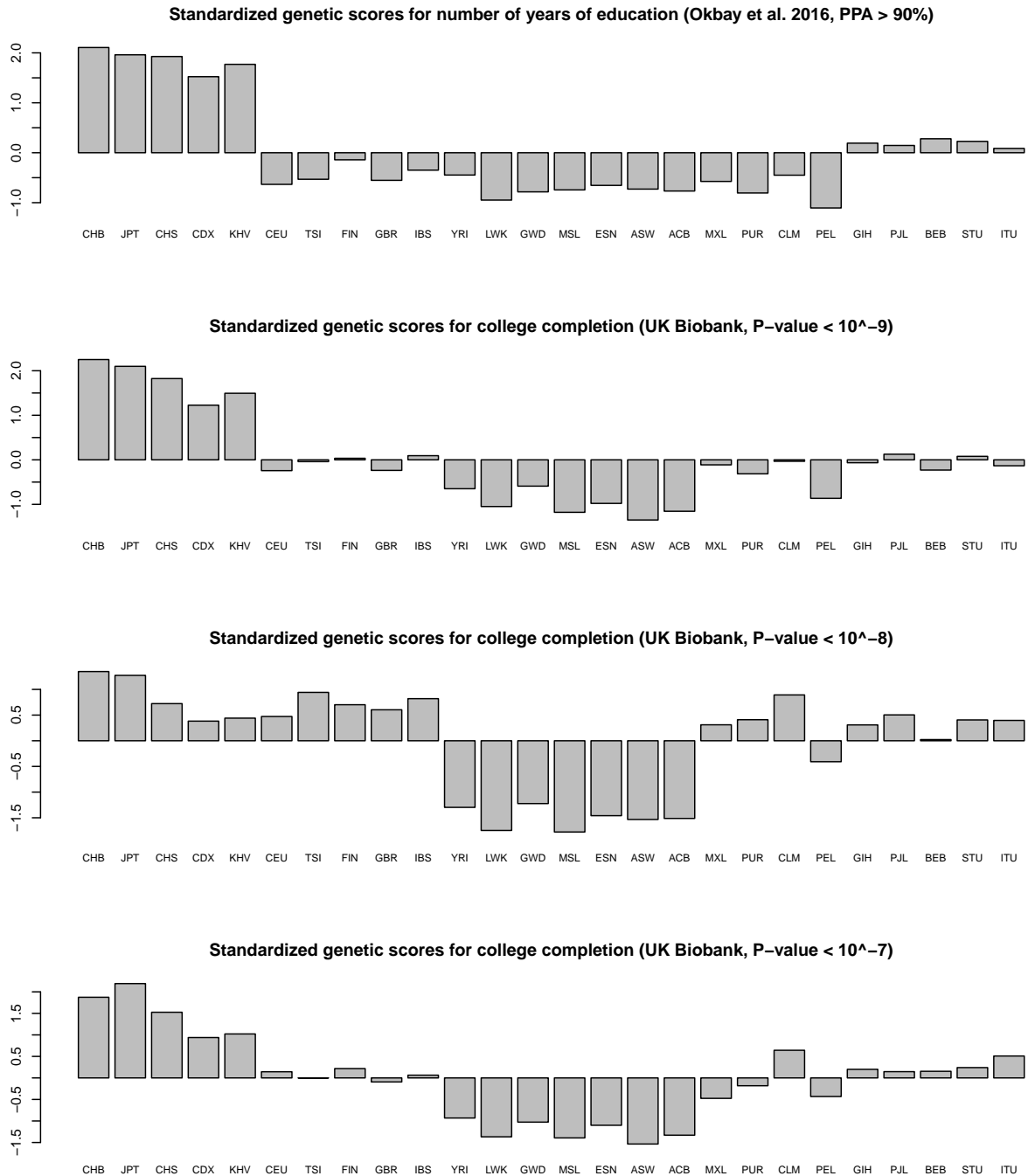
Figure S47: We compared the standardized population genetic scores using the ref. [46] GWAS data for number of years of education - looking at LD blocks with a posterior probability of association (PPA) > 90% (top panel), with the standardized population genetic scores using the Neale lab GWAS data performed on the UK Biobank, for completion of college / university degree (lower panels). We selected the SNP with the lowest P-value per LD block, and then used different P-value cutoffs to build the score: 10^{-9} , 10^{-8} , 10^{-7} .
