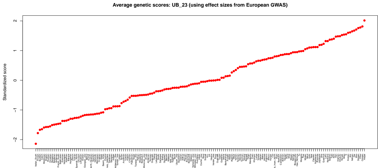
Figure S51: Standardized average genetic scores for self-reported unibrow of each of the populations in the Human Origins SNP chip dataset. Note that the scores are built using effect sizes from a European GWAS, so the accuracy of the score will likely decrease with increasing genetic distance from European populations.
