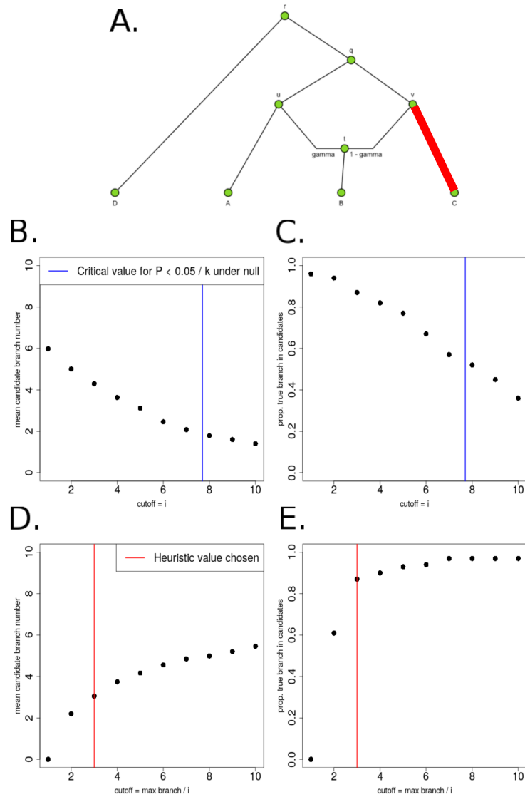
Figure S60: A. We produced 100 simulations of polygenic adaptation in a terminal branch of a graph (C-v), each with 400 SNPs and \alpha = 0.2 . All branches had drift lengths equal to 0.05 B. We tested various cutoffs for Q_B and plotted the average number of candidate branches that passed the cutoff, over all simulations. The blue line is the X_1^2 cutoff corresponding to P = 0.05/k , where k is the number of branches in the graph, under the null hypothesis of no selection. C. For each of the same cutoffs, we also plotted the proportion of simulations in which the true selected branch was among the candidate branches. D. Instead of testing constant values for the Q_B cutoff, we chose the cutoff to be the maximum branch statistic in each simulation, divided by i , and tested various values of i . We plotted the average number of candidate branches that passed the cutoff, over all simulations. E. For the same cutoff method as in panel D, we plotted the proportion of simulations in which the true selected branch was among the candidate branches. For simulations and applications to real data, we chose a heuristic value ( i=3 , red line).
