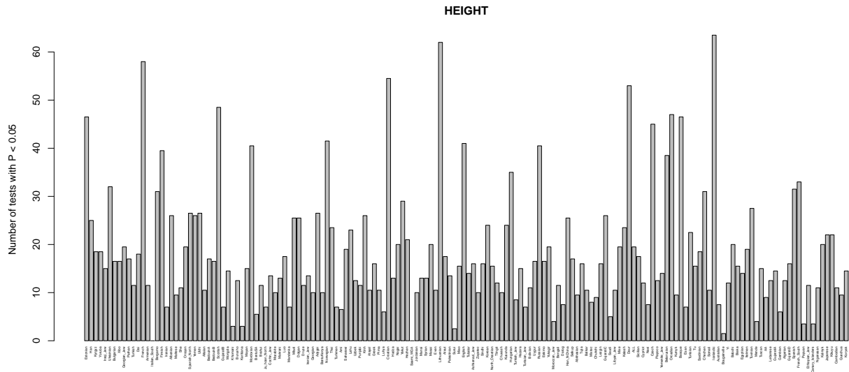
Figure S44: This barplot shows, for each panel, the number of two-tailed binomial tests for systematic allele frequency differences in the sign of the effect size estimate of variants associated with height with P-values < 0.05 , which involve that panel as a member of the pair. We tested all panels from the Lazaridis et al. (2014) dataset.
