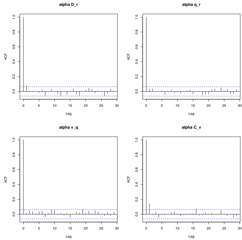
Figure S52: Auto-correlation plots for \alpha parameters of simulation 1 of Figure S5. The rest of the \alpha parameters did not pass the Q_B cutoff and were therefore set to a fixed value of 0 throughout the chain.
