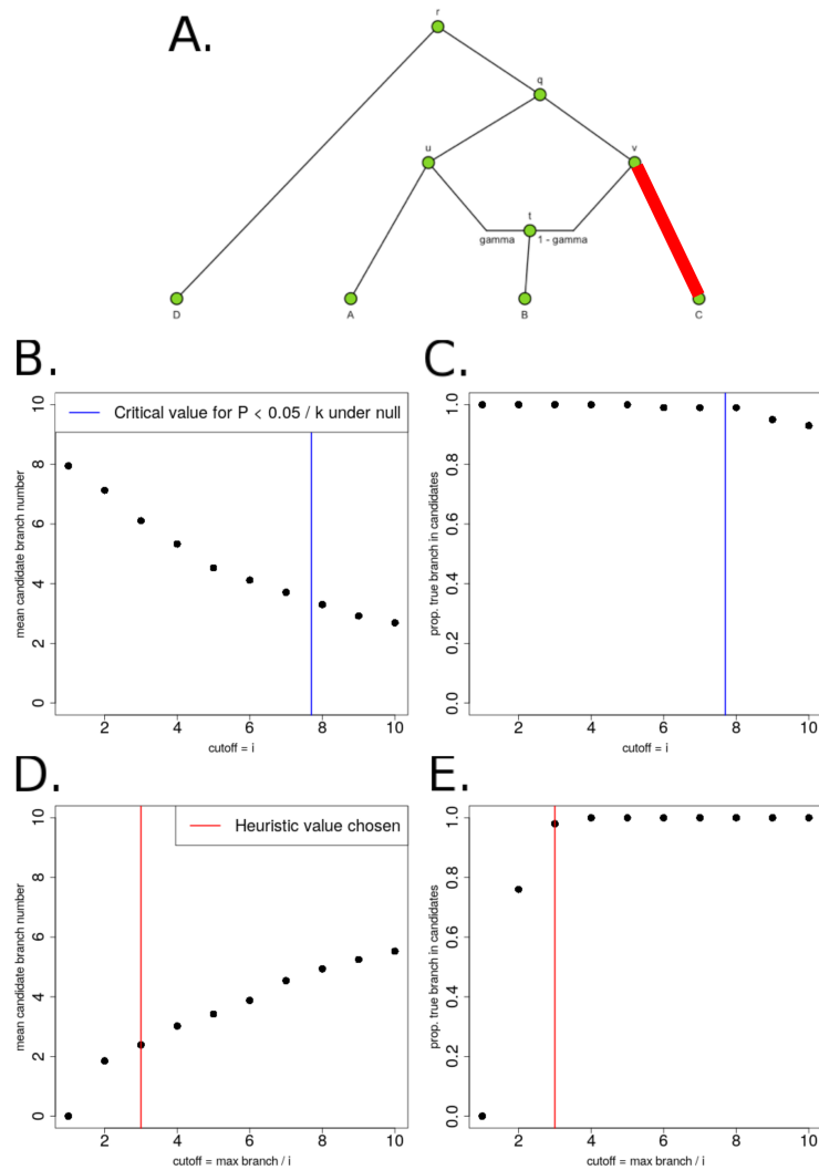
Figure S58: A. We produced 100 simulations of polygenic adaptation in a terminal branch of a graph (C-v), each with 400 SNPs and \alpha = 0.2 . All branches had drift lengths equal to 0.02 B. We tested various cutoffs for Q_B and plotted the average number of candidate branches that passed the cutoff, over all simulations. The blue line is the X_1^2 cutoff corresponding to P = 0.05/k , where k is the number of branches in the graph, under the null hypothesis of no selection. C. For each of the same cutoffs, we also plotted the proportion of simulations in which the true selected branch was among the candidate branches. D. Instead of testing constant values for the Q_B cutoff, we chose the cutoff to be the maximum branch statistic in each simulation, divided by i , and tested various values of i . We plotted the average number of candidate branches that passed the cutoff, over all simulations. E. For the same cutoff method as in panel D, we plotted the proportion of simulations in which the true selected branch was among the candidate branches. For simulations and applications to real data, we chose a heuristic value ( i=3 , red line).
