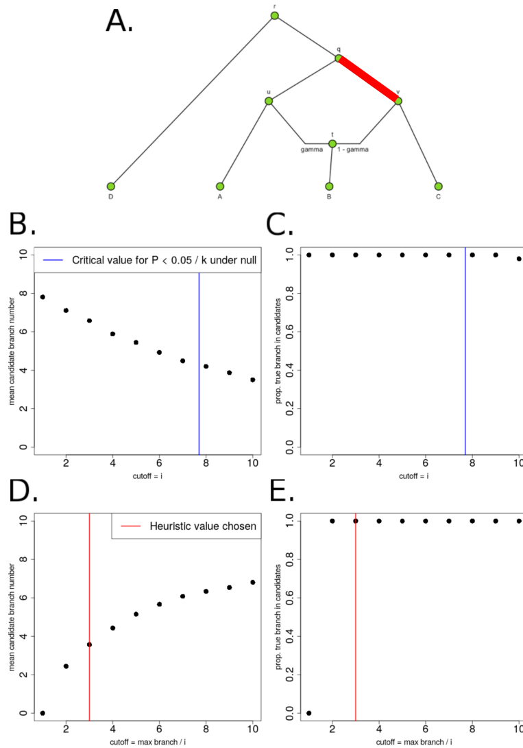
Figure S57: A. We produced 100 simulations of polygenic adaptation in an internal branch of a graph ( v - q ), each with 400 SNPs and \alpha = 0.2 . All branches had drift lengths equal to 0.02 B. We tested various cutoffs for Q_B and plotted the average number of candidate branches that passed the cutoff, over all simulations. The blue line is the \chi^2_1 cutoff corresponding to P = 0.05/k , where k is the number of branches in the graph, under the null hypothesis of no selection. C. For each of the same cutoffs, we also plotted the proportion of simulations in which the true selected branch was among the candidate branches. D. Instead of testing constant values for the Q_B cutoff, we chose the cutoff to be the maximum branch statistic in each simulation, divided by i , and tested various values of i . We plotted the average number of candidate branches that passed the cutoff, over all simulations. E. For the same cutoff method as in panel D, we plotted the proportion of simulations in which the true selected branch was among the candidate branches. For simulations and applications to real data, we chose a heuristic value ( i=3 , red line).
