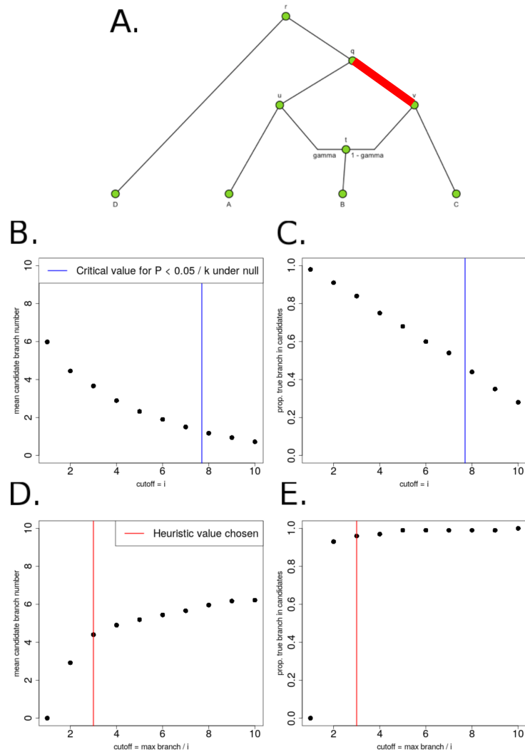
Figure S53: A. We produced 100 simulations of polygenic adaptation in an internal branch of a graph ( v - q ), each with 400 SNPs and \alpha = 0.1 . All branches had drift lengths equal to 0.02 B. We tested various cutoffs for Q_B and plotted the average number of candidate branches that passed the cutoff, over all simulations. The blue line is the \chi^2_1 cutoff corresponding to P = 0.05/k , where k is the number of branches in the graph, under the null hypothesis of no selection. C. For each of the same cutoffs, we also plotted the proportion of simulations in which the true selected branch was among the candidate branches. D. Instead of testing constant values for the Q_B cutoff, we chose the cutoff to be the maximum branch statistic in each simulation, divided by i , and tested various values of i . We plotted the average number of candidate branches that passed the cutoff, over all simulations. E. For the same cutoff method as in panel D, we plotted the proportion of simulations in which the true selected branch was among the candidate branches. For simulations and applications to real data, we chose a heuristic value ( i=3 , red line).
