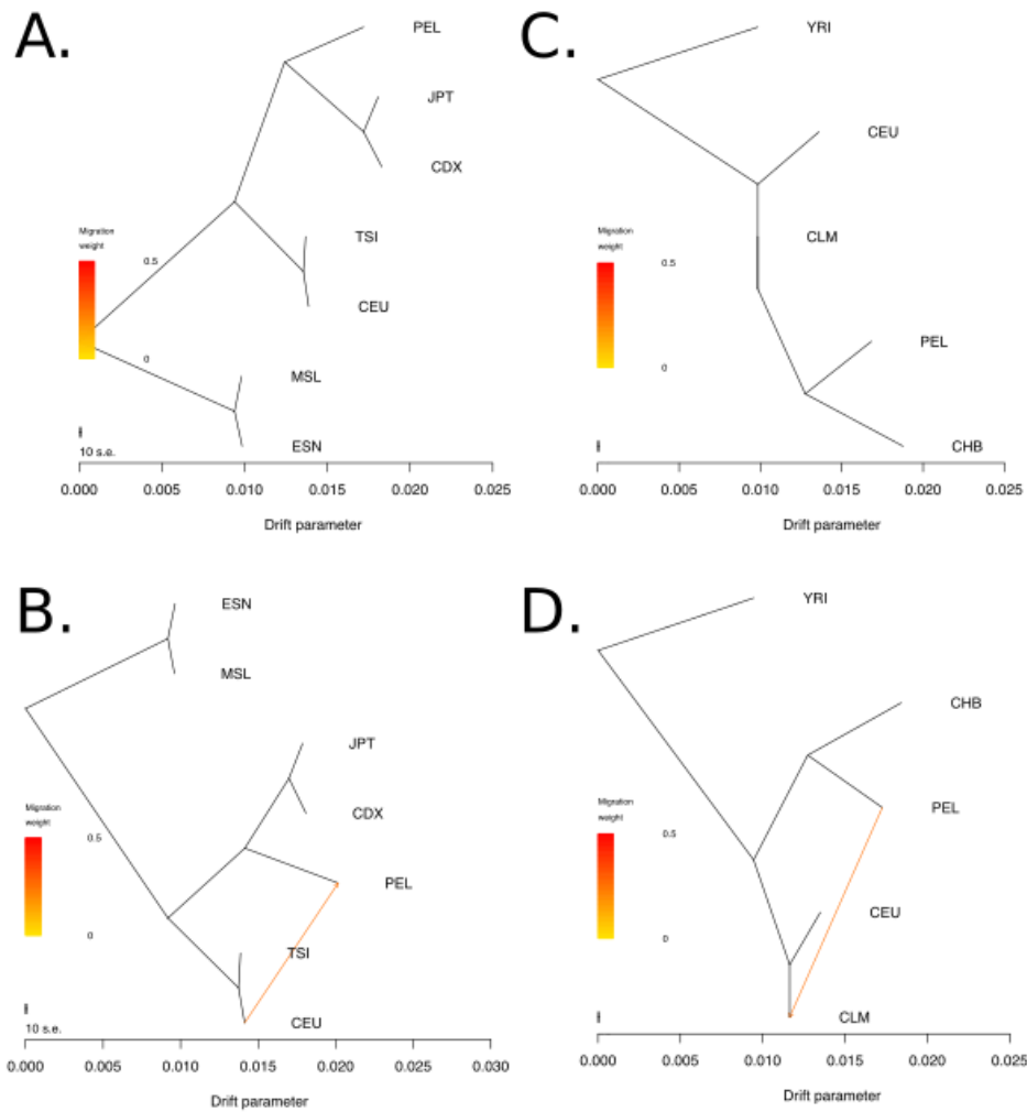
Figure S61: A. Topology inferred by TreeMix when forcing no admixture events and inputting the following populations from the 1000 Genomes Project: MSL, ESN, CDX, JPT, CEU, TSI and PEL. B. Topology inferred by TreeMix when inputting the same populations as in panel A, but forcing 1 migration event. C. Topology inferred by TreeMix when forcing no admixture events and inputting the following populations from the 1000 Genomes Project: YRI, CEU, CHB, PEL, CLM. D. Topology inferred by TreeMix when inputting the same populations as in panel C, but forcing 1 migration event. The trees were rooted such that the African populations were an outgroup to the rest of the populations. We note that the drift parameters outputted by TreeMix - unlike those outputted by MixMapper - are a product of the drift parameter that we use in PolyGraph and the average over the inferred heterozygosities at each branch ancestral node, computed over all SNPs used to produce the TreeMix graph.
