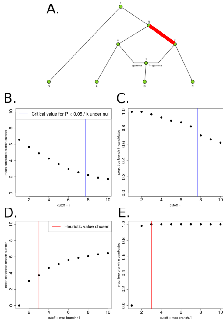
Figure S59: A. We produced 100 simulations of polygenic adaptation in an internal branch of a graph ( v - q ), each with 400 SNPs and \alpha = 0.2 . All branches had drift lengths equal to 0.05 B. We tested various cutoffs for Q_B and plotted the average number of candidate branches that passed the cutoff, over all simulations. The blue line is the \chi^2_1 cutoff corresponding to P = 0.05/k , where k is the number of branches in the graph, under the null hypothesis of no selection. C. For each of the same cutoffs, we also plotted the proportion of simulations in which the true selected branch was among the candidate branches. D. Instead of testing constant values for the Q_B cutoff, we chose the cutoff to be the maximum branch statistic in each simulation, divided by i , and tested various values of i . We plotted the average number of candidate branches that passed the cutoff, over all simulations. E. For the same cutoff method as in panel D, we plotted the proportion of simulations in which the true selected branch was among the candidate branches. For simulations and applications to real data, we chose a heuristic value ( i=3 , red line).
