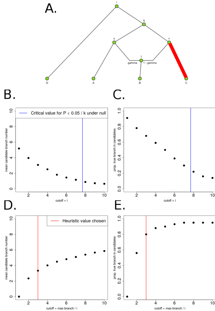
Figure S54: A. We produced 100 simulations of polygenic adaptation in a terminal branch of a graph (C-v), each with 400 SNPs and \alpha = 0.1 . All branches had drift lengths equal to 0.02 B. We tested various cutoffs for Q_B and plotted the average number of candidate branches that passed the cutoff, over all simulations. The blue line is the X_1^2 cutoff corresponding to P = 0.05/k , where k is the number of branches in the graph, under the null hypothesis of no selection. C. For each of the same cutoffs, we also plotted the proportion of simulations in which the true selected branch was among the candidate branches. D. Instead of testing constant values for the Q_B cutoff, we chose the cutoff to be the maximum branch statistic in each simulation, divided by i , and tested various values of i . We plotted the average number of candidate branches that passed the cutoff, over all simulations. E. For the same cutoff method as in panel D, we plotted the proportion of simulations in which the true selected branch was among the candidate branches. For simulations and applications to real data, we chose a heuristic value ( i=3 , red line).
