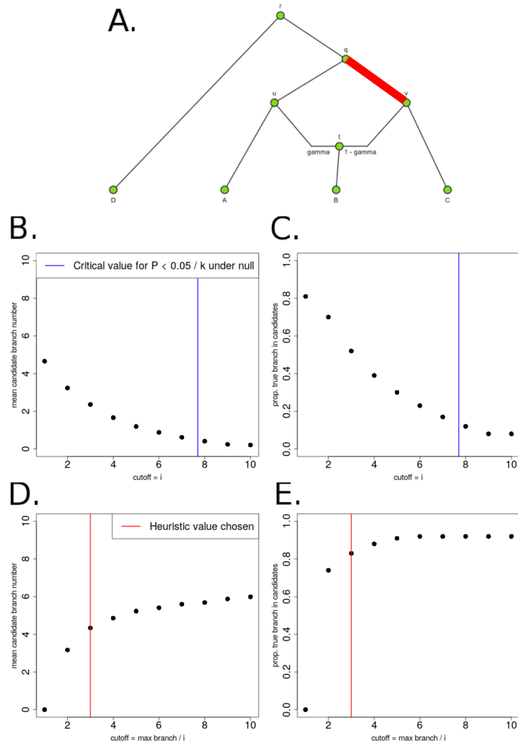
Figure S55: A. We produced 100 simulations of polygenic adaptation in an internal branch of a graph ( v - q ), each with 400 SNPs and \alpha = 0.1 . All branches had drift lengths equal to 0.05 B. We tested various cutoffs for Q_B and plotted the average number of candidate branches that passed the cutoff, over all simulations. The blue line is the \chi^2_1 cutoff corresponding to P = 0.05/k , where k is the number of branches in the graph, under the null hypothesis of no selection. C. For each of the same cutoffs, we also plotted the proportion of simulations in which the true selected branch was among the candidate branches. D. Instead of testing constant values for the Q_B cutoff, we chose the cutoff to be the maximum branch statistic in each simulation, divided by i , and tested various values of i . We plotted the average number of candidate branches that passed the cutoff, over all simulations. E. For the same cutoff method as in panel D, we plotted the proportion of simulations in which the true selected branch was among the candidate branches. For simulations and applications to real data, we chose a heuristic value ( i=3 , red line).
