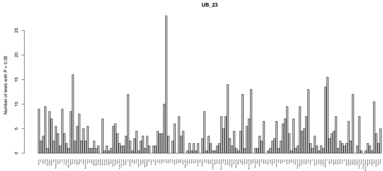
Figure S46: This barplot shows, for each panel, the number of two-tailed binomial tests for systematic allele frequency differences in the sign of the effect size estimate of variants associated with self-reported unibrow with P -values < 0.05 , which involve that panel as a member of the pair. We tested all panels from the Lazaridis et al. (2014) dataset.
