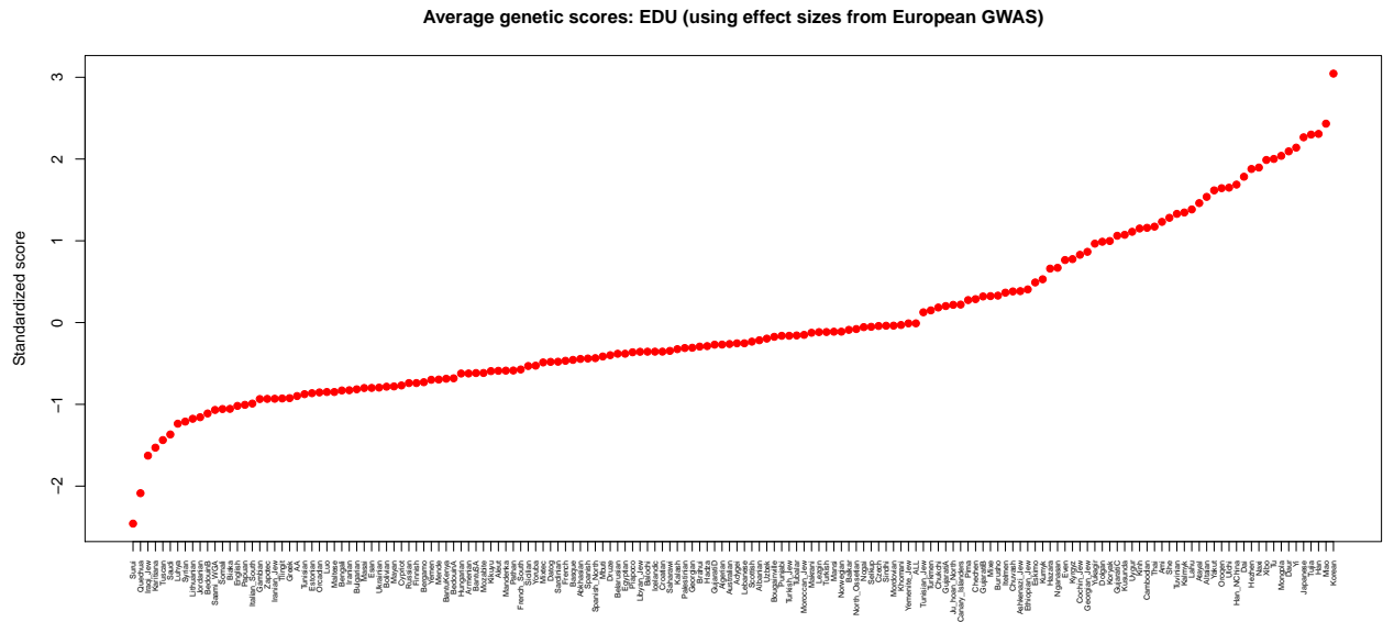
Figure S49: Standardized average genetic scores for educational attainment of each of the populations in the Human Origins SNP chip dataset. Note that the scores are built using effect sizes from a European GWAS, so the accuracy of the score will likely decrease with increasing genetic distance from European populations.
