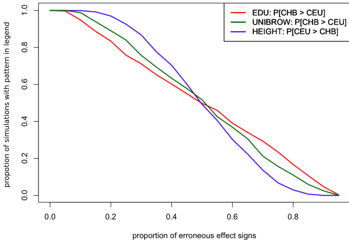
Figure S36: We simulated different proportions of incorrectly assigned signs for the effect size estimates of trait-associated SNPs. We then assessed - for each proportion - how often we could recreate the inequality relationship observed between the polygenic scores for CHB and CEU built using the trait-associated SNPs of the three traits with strongest evidence for polygenic adaptation: height, educational attainment and self-reported unbrow. The observed inequality relationship for educational attainment and unbrow is Poly_{CHB} > Poly_{CEU} , where Poly_X is the polygenic score for panel X. The observed inequality relationship for height is the reverse: Poly_{CEU} > Poly_{CHB} . We used 10,000 simulations for each sign misassignment scenario.
