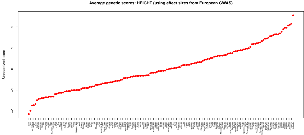
Figure S50: Standardized average genetic scores for height of each of the populations in the Human Origins SNP chip dataset. Note that the scores are built using effect sizes from a European GWAS, so the accuracy of the score will likely decrease with increasing genetic distance from European populations.
