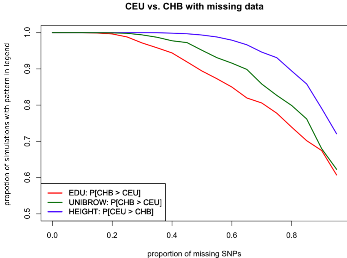
Figure S35: We simulated different proportions of missing trait-associated SNPs ( x -axis). We then assessed - for each proportion - how often we could recreate the inequality relationship observed between the polygenic scores for CHB and CEU built using the trait-associated SNPs of the three traits with strongest evidence for polygenic adaptation: height, educational attainment and self-reported unbrow. The observed inequality relationship for educational attainment and unbrow is Poly_{CHB} > Poly_{CEU} , where Poly_X is the polygenic score for panel X. The observed inequality relationship for height is the reverse: Poly_{CEU} > Poly_{CHB} . We used 10,000 simulations for each missing data scenario.
