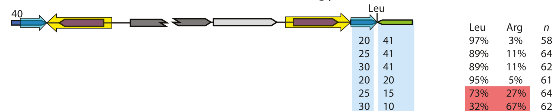
Fig 6. Alternative strategies for generating point mutations with DIRex. (A) Schematic view of the recombineering used for these tests. The recipient strain carries a L169R mutation in hisA , rendering it His - (but Trp + ). The incoming PCR fragments are designed to repair this mutation, making the wanted transformants (after segregation of the cassette) His + (but Trp - ). (B) Constructs with the mutation in the middle of the DRs. The site of the mutation is indicated in both DRs with asterisks. "Leu" and "Arg" below the DRs indicate which allele was present in the corresponding PCR product. In the table to the right, "Leu" indicates the fraction of transformants that only segregated to the L169 (wanted) allele, "Both" the fraction of transformants that segregated to both alleles, and "Arg" the fraction of transformants that only segregated to the R169 (parental) allele. (C) Constructs with the mutation next to the ter proximal DR. "o" and "p" indicate presence of a 5'-hydroxyl or 5'-phosphate, respectively, at the indicated end of the PCR fragment. (D) Constructs with the mutation next to the ori
