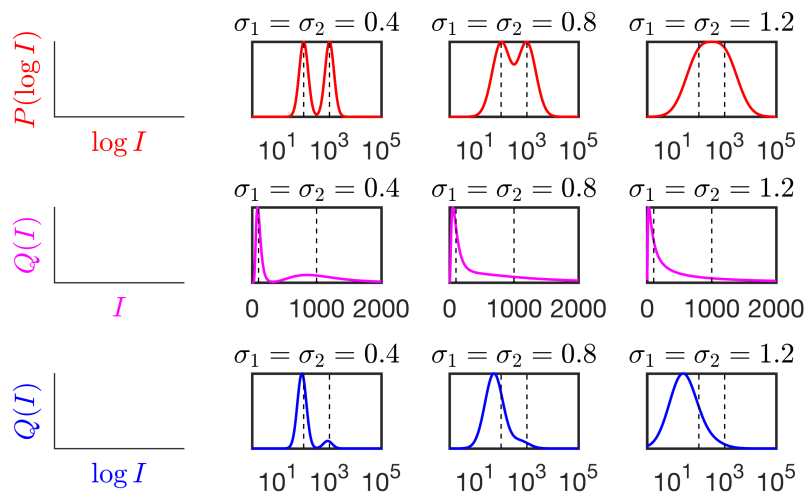
Fig 1. Log-normal mixture showing the mismatch in the number of peaks. Top row, red: P(\log I) vs. \log I normalized to maximum probability. Middle row, magenta: Q(I) vs. I normalized to maximum probability, and plotted on a narrower range. Bottom row, blue: Q(I) vs. \log I normalized to maximum probability, rescaling the x-axis as in Ref. (6). In the central column where \sigma_1 = \sigma_2 = 0.8 , P(\log I) shows explicit bimodality whereas Q(I) is unimodal. Right column: in this case, the variance \sigma^2 is large enough (see Eq. 4) that P(\log I) has only one mode even though it is modeled as a mixture. In all cases: I_1 = 100 , I_2 = 1000 , \alpha = 0.5 varying \sigma_{1,2} = \{0.4, 0.8, 1.2\} (left to right columns, respectively). Leftmost column shows axes.
