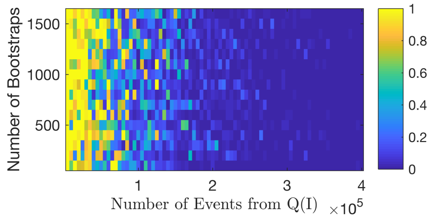
Fig 7. Testing Hartigan’s p-value p_u for unimodality on a weakly bimodal log-normal mixture. The heat-map shows p_u as a function of the number of bootstrap tests and number of events in each test, for \sigma_1 = 0.4 and \sigma_2 = 0.8 as in Fig. 2(top,middle). With less than \sim 10^5 events, Hartigan’s test for this case may misidentify the number of peaks.
