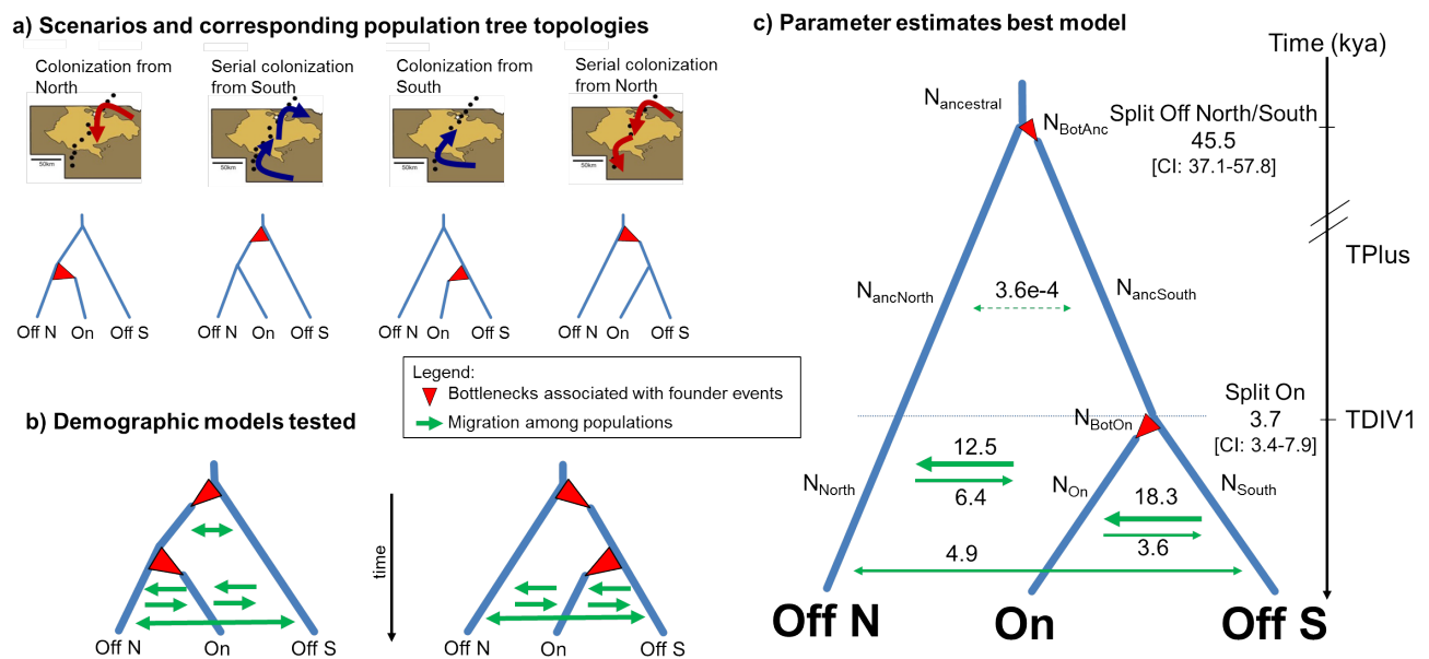
Supplementary Figure 2. Demographic modeling favors colonization from the south. (a) Four scenarios were tested and the corresponding three-population model tree topologies are provided. The three samples correspond to populations north of the Sand Hills (Off N), on the Sand Hills (On), and south of the Sand Hills (Off S). Although alternative scenarios might have identical population trees, they can be distinguished as founder events associated with the colonization of the Sand Hills are expected to occur on different lineages. (b) Demographic models tested with two topologies, allowing for up to two bottlenecks associated with the population split, and gene flow among populations. Under this modeling framework, we can distinguish among scenarios with the same tree topology by inferring the strength of the bottlenecks associated with the split of the Sand Hills populations (indicated as red arrows), representing potential founder events related with the colonization of the Sand Hills. For instance, for the tree topology ((Off N, On), Off S), if inferred parameters indicate a stronger bottleneck associated with the Sand Hills (“On”), it would support a colonization from the north scenario, whereas a stronger bottleneck associated with the split of the ancestor of “Off N” and “On” would suggest a serial colonization from the south. (c) Parameter estimates under the best model, supporting a southern colonization route. Parameter estimates for scaled immigration rates 2Nm (i.e., average number of immigrants per generation) are shown above or below corresponding arrows, and the time of events (given in thousand years (kya)) is indicated at the nodes, assuming 2.5 generations per year and a mutation rate of 3.67 \times 10^{-8} per site per generation. Parameter tags are indicated next to each corresponding parameter. Demographic modeling was based on the three-dimensional minor allele frequency spectrum (3D MSFS), considering models with three populations. The 3D folded SFS was generated by dividing the data set into blocks of 1.5kb, sampling ten individuals for each block from each population without missing data - resulting in a 3D folded SFS with 140,358 SNPs.
