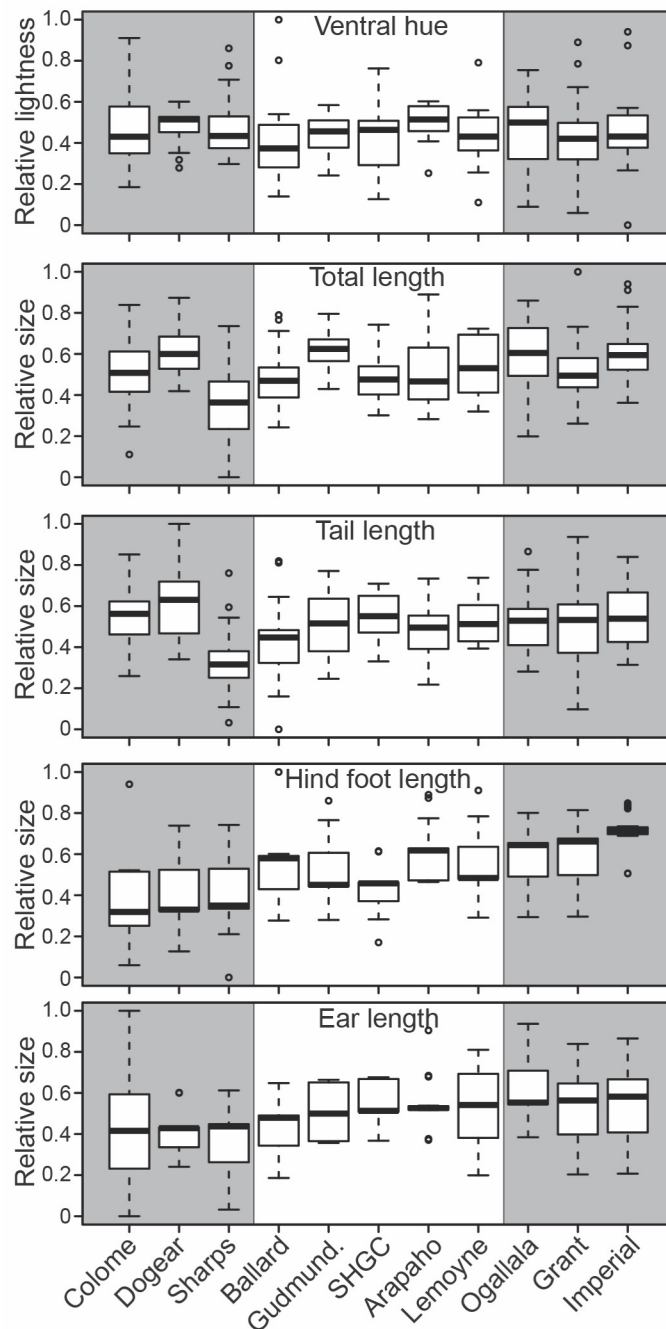
Supplemental Figure 11. Ventral hue and non-color traits are not significantly different on and off the Sand Hills. Box plots for each sampling site were produced using scaled (range: 0-1), normal-quantile transformed values for: ventral hue (PC4), total body length, tail length, hind foot length, and ear length. In all plots, higher values correspond to lighter/brighter color or longer lengths. Grey shading indicates non-Sand Hills sites. Ventral hue did not differ significantly between habitats (on vs. off Sand Hills) or among sites ( P > 0.05 ). All four length traits differed significantly among sites nested within habitats, but not among habitats.
