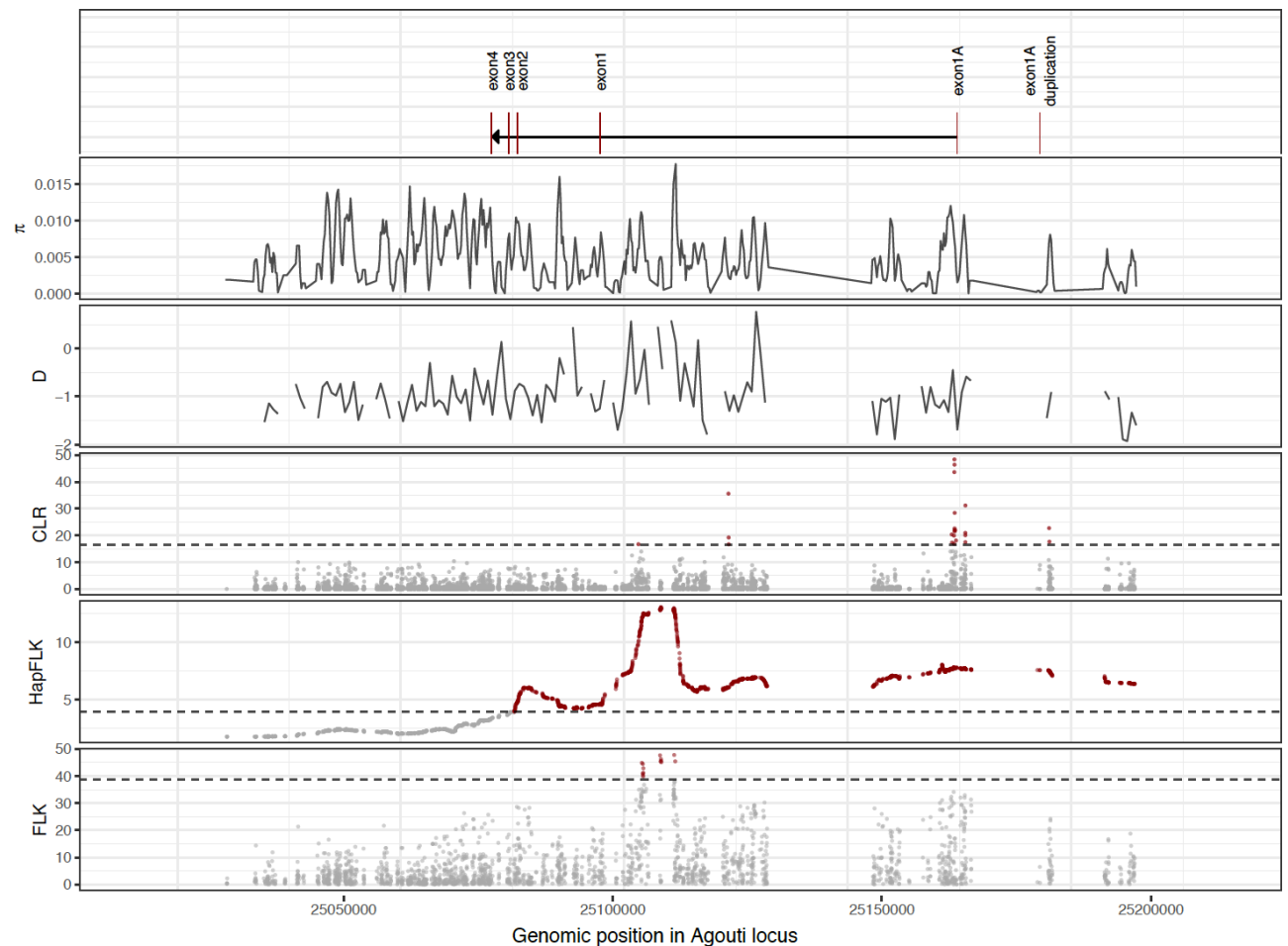
Supplementary Figure 10. Comparison of tests of neutrality and selection across the Agouti locus. From the top, the exon structure, pairwise differences, Tajima's D , CLR test, HapFLK, and FLK. The dashed lines indicate the significance threshold using parametric bootstrapping of the best-fitting demographic model.
