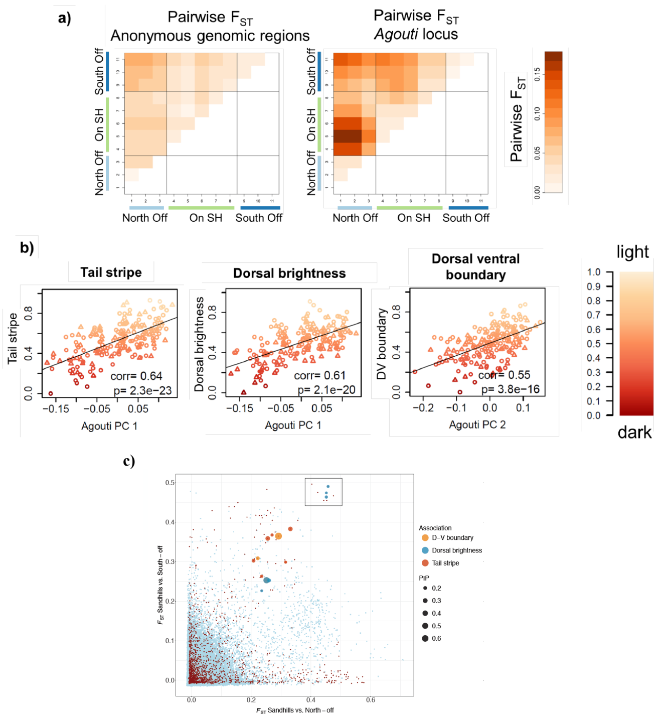
Supplementary Figure 5. Comparison of genetic differentiation for random background genomic regions and Agouti . (a) F_{ST} for samples along the transect. At the Agouti locus, higher F_{ST} values are observed, particularly for comparisons between samples On (green) and Off (blue) of the Sand Hills. (b) Genetic differentiation at Agouti is correlated with phenotypic trait values. PC1 correlates with tail stripe and dorsal brightness, whereas PC2 correlates with the dorsal ventral boundary, in agreement with Linnen et al. 2013 (color-coded with darker phenotypes in darker shades). Circles represent males, and triangles females. (c) The x-axis gives F_{ST} values for On vs. North, and the y-axis gives values for On vs. South. Points highlighted by a square correspond to the highest peak of differentiation. For SNPs with F_{ST} values above 0.2, their estimated contribution to the phenotypes considered in the association study are indicated by dot size (PIP > 0.15).
