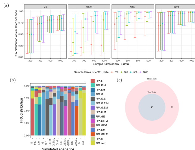
Figure 2. Results from simulations under colocalization/non-colocalization scenarios (A-B), and results from real data application (C). A. Simulations under different sample sizes for all scenarios in moloc of three traits (GWAS, eQTL, mQTL). The y axis shows the median, 10% and 90% quantile of the distribution of posterior probabilities (“PPA”), which supports each of our scenarios of interest. Combined scenarios include gene-methylation pairs or genes that reach a posterior probability of GEM \geq 80\% , or + GEM \geq 80\% , or GE \geq 80\% . All cases include 10,000 individuals in the GWAS dataset. The variance explained by the trait was set to 0.01 for GWAS (1%), and to 0.1 (10%) for the eQTL and mQTL. B. Posterior probabilities from simulations using a sample size of 10,000 individuals for GWAS trait (denoted as G), 300 for eQTL trait (denoted as E), and 300 for mQTL trait (denoted as M). X-axis shows all 15 simulated scenarios, e.g. G.E.M, three different causal variants for each of the three traits. Y-axis shows the distribution of posterior probabilities under the simulated scenario. The height of the bar represents the mean of the PPA for each configuration across simulations. C. Venn diagram comparing number of colocalization of two traits ( coloc\ PPA \geq 80\% ) with three traits ( moloc\ PPA\ GE + GEM + GEM ) in simulations with one causal variant shared between all the three traits (GEM). Results include 887 out of 1,000 simulations passing 80% threshold for colocalization.
