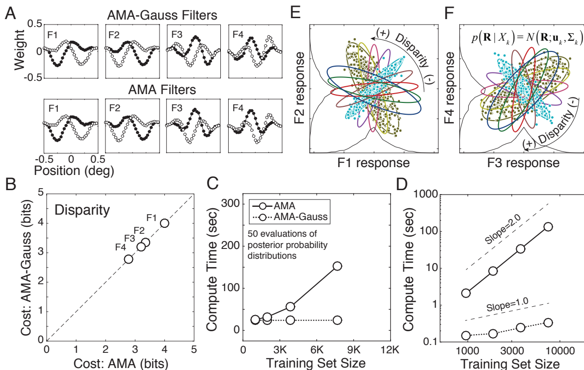
Figure 6: Disparity estimation task: filters, cost, compute time, and class-conditional response distributions. A AMA-Gauss and AMA filters for estimating disparity from natural stereo-images (-15 to +15 arcmin). B-F Caption format same as Fig. 5.B-F.
