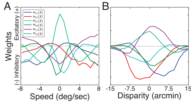
Figure 9: Quadratic pooling weights for computing the likelihood. Weights on squared and sum-squared filter responses ( w_{ii}(X) and w_{ij}(X) ) as a function of the latent variable. Weights on the linear filter responses are all approximately zero and are not shown. A Weights for speed estimation task. B Weights for disparity estimation task. Weights on squared responses are at maximum magnitude when the variance of the corresponding filter responses are at minimum. Weights on sum-squared responses are at maximum magnitude for latent variables yielding maximum response covariance (see Figs. 5.EF and 6.EF).
