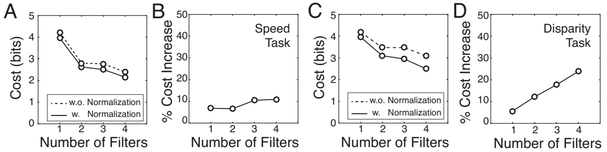
Figure 8: Decoding performance with and without contrast normalization. A Contrast normalization decreases decoding cost for the speed estimation task. B Percentage increase in cost without contrast normalization. C-D Same as A-B, but for the disparity estimation task. The same result holds for different cost functions (e.g. squared error) and larger number of filters. If eight filters are used in the disparity task, failing to contrast normalize can decrease performance by \sim 40\% .
