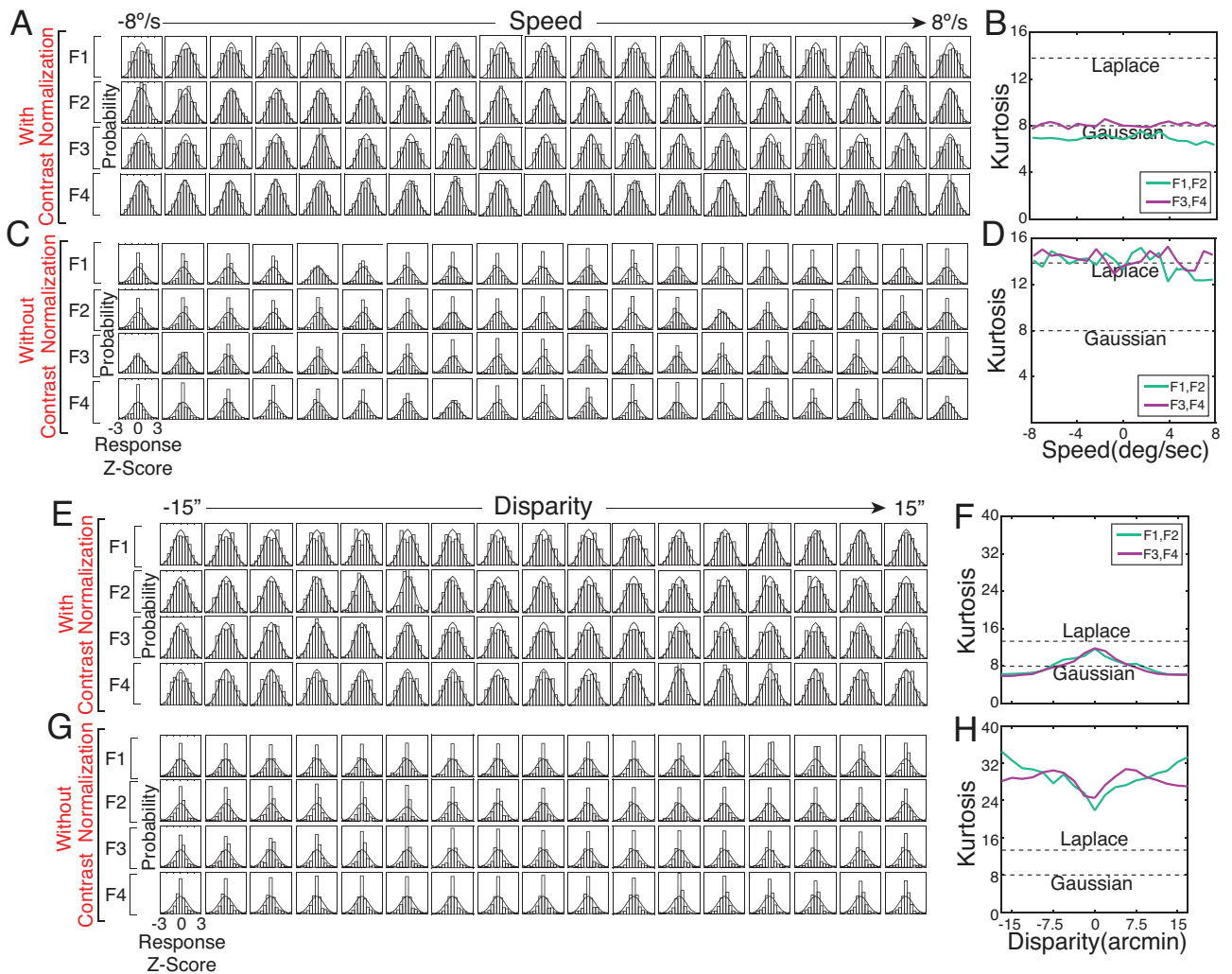
Figure 7: Filter responses with and without contrast normalization. A Class-conditional filter response distributions \mathcal{P}(R_t|X_u) to contrast-normalized stimuli for each individual filter and each level of the latent variable in the speed estimation task. For visualization, responses are transformed to Z -scores by subtracting off the mean and dividing by the standard deviation. Gaussian probability density is overlaid for purposes of comparison. B Kurtosis of the two-dimensional conditional response distributions from filters 1 and 2 (violet; also see Fig. 5.E) and filters 3 and 4 (green; also see Fig. 5.F) for all levels of the latent variable. A two-dimensional Gaussian has a kurtosis of 8.0. Kurtosis was estimated by fitting a multidimensional generalized Gaussians via maximum likelihood methods. C,D Same as A,B but without contrast normalization. E-H Same as A-D, but for the task of disparity estimation.
