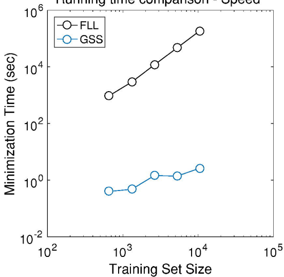
Running time comparison - Speed
