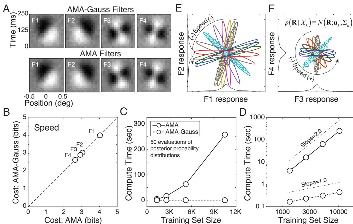
Figure 5: Speed estimation task: filters, cost, compute time, and class-conditional response distributions. A AMA-Gauss and AMA filters for estimating speed (-8 to +8 deg/sec) from natural image movies are nearly identical; \rho > 0.96 for all filters. B The cost for all the filters for both the models is identical. C Compute time for fifty evaluations of the posterior probability distribution is linear with AMA-Gauss, and quadratic with the full AMA model, in the training set size. D Same data as in C but on log-log axes. E,F Joint filter responses, conditioned on each level of the latent variable, are approximately Gaussian (also see below). Different colors indicate different speeds. Individual symbols represent responses to individual stimuli. Thin black curves show that the filter response distributions, marginalized over the latent variable \mathcal{P}(R) = \sum_{u=1}^{N_{lvl}} \mathcal{P}(R|X_u)\mathcal{P}(X_u) , are heavier-tailed than Gaussians (see Sections 3, 4)
