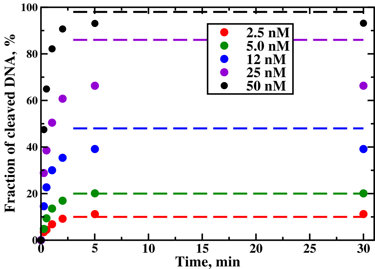
Figure 2: Comparison between experimental measurements (filled circles) and theoretical predictions (dashed lines) for the fraction of cleaved DNA as a function of time. The experimental data are taken from Ref.(5).
