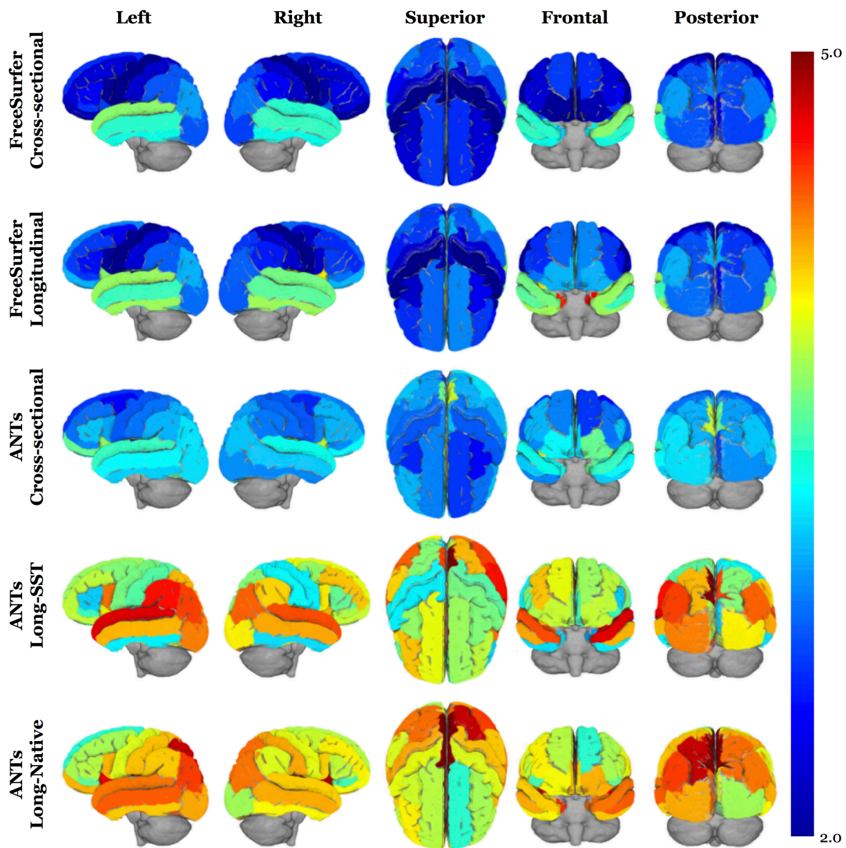
Figure 7: 3-D volumetric rendering of the regional variance ratio values on the generated ADNI template. The higher variance ratios indicate greater between-subject to within-subject variability.
