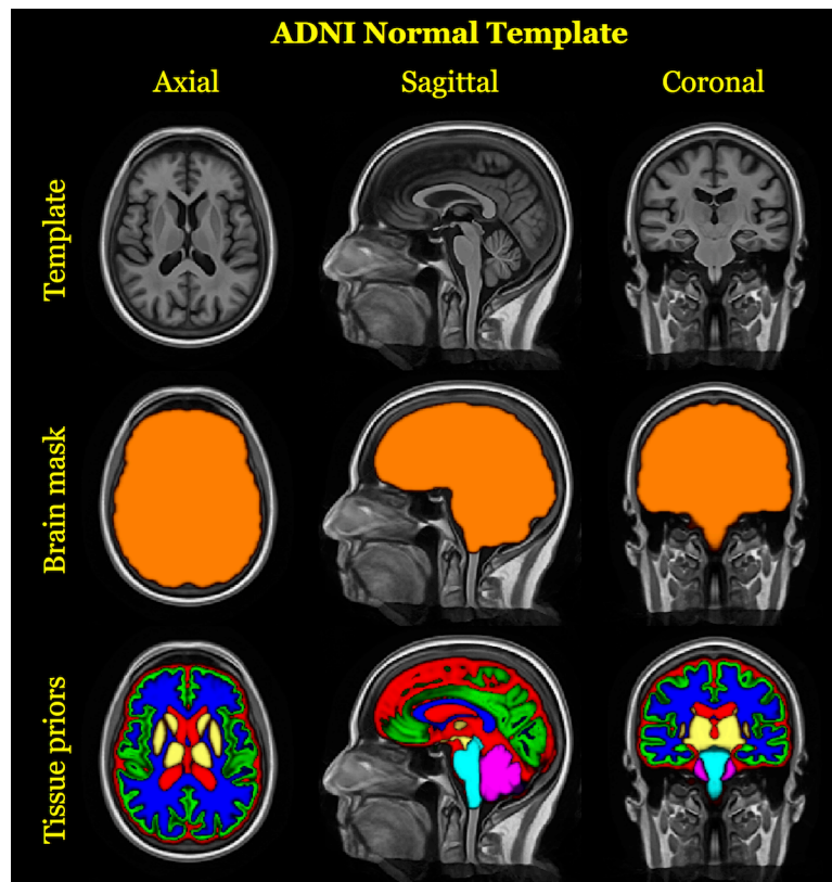
Figure 4: Top row: Canonical views of the template created from 52 cognitively normal subjects of the ADNI-1 database. The prior probability mask for the whole brain (middle row) and the six tissue priors (bottom row) are used to “seed” each single-subject template for creation of a probabilistic brain mask and probabilistic tissues priors during longitudinal processing.
