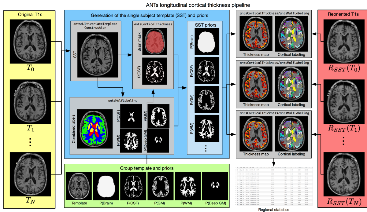
Figure 3: Diagrammatic illustration of the ANTs longitudinal cortical thickness pipeline for a single subject with N time points. From the N original T1-weighted images (left column, yellow panel) and the group template and priors (bottom row, green panel), the single-subject template (SST) and auxiliary prior images are created (center, blue panel). These subject-specific template and other auxiliary images are used to generate the individual time-point cortical thickness maps, in the individual time point’s native space (denoted as “Longitudinal-native” in the text). Optionally, one can rigidly transform the time-point images prior to segmentation and cortical thickness estimation (right column, red panel). This alternative processing scheme is referred to as “Longitudinal-SST”. For regional thickness values, regional labels are propagated to each image using a given atlas set (with cortical labels) and joint label fusion.
