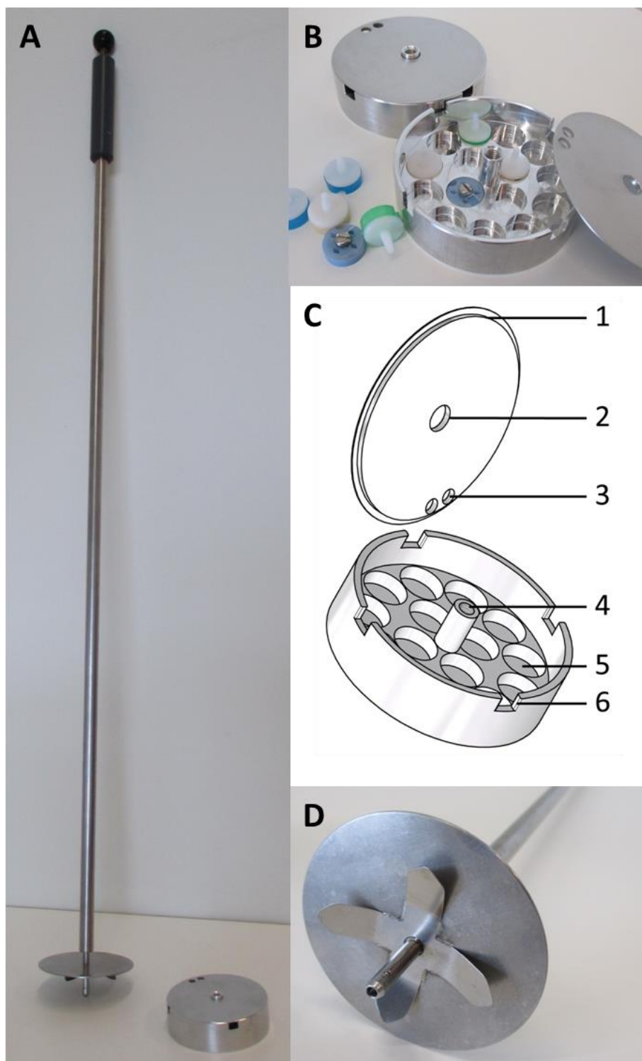
Figure 1. The cryo-storage system designed and developed for the preservation of cryo-EM samples
