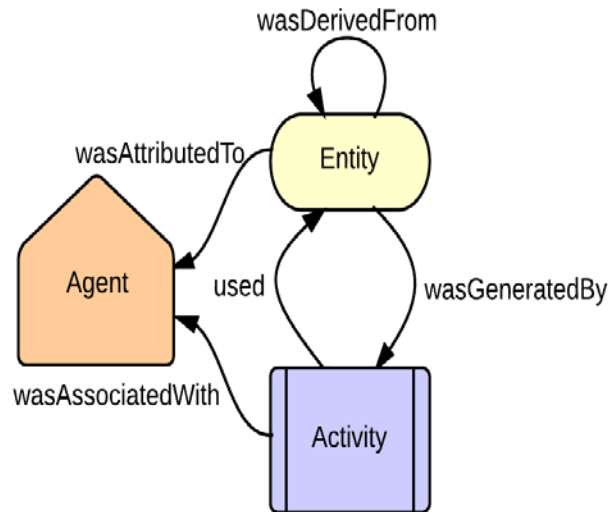
Fig 2. W3C Provenance Specification used in FHIR and ROs. Adapted from http://www.w3.org/TR/prov-primer/
