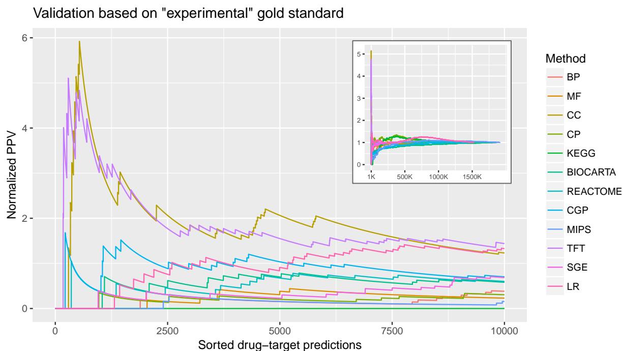
Figure 3: Validation of Gene2Drug against the STITCH experimental gold-standard. Only drug-target pairs present in STITCH and supported by experimental evidence were included in this gold-standard (refer to Tab. 2 for additional gold-standards). For each one of the 12 methods, we obtained a list of drug-target pairs ranked according to their weight as computed by the method. The Positive Predictive Value TP/(TP + FP) was computed for each rank, according to the STITCH experimental gold-standard, and divided by the "random" PPV obtained by ranking drug-target pairs randomly (Normalised PPV). Each line represents the PPV of one of the 12 methods as indicated in the legend for the top 10,000 drug-target pairs. Inset: PPV versus drug-targets but this time showing the PPV for all of the possible drug-target pairs, which vary according to the chosen database (BP: 1,853,544; MF: 1,864,016; CC: 1,233,078; CP: 1,117,886; KEGG: 1,127,049; BIOCARTA: 1,848,308; REACTOME: 1,424,192; CGP: 1,479,170; MIPS: 1,916,376; TFT: 442,442; SGE: 335,104; LR: 1,524,985).
