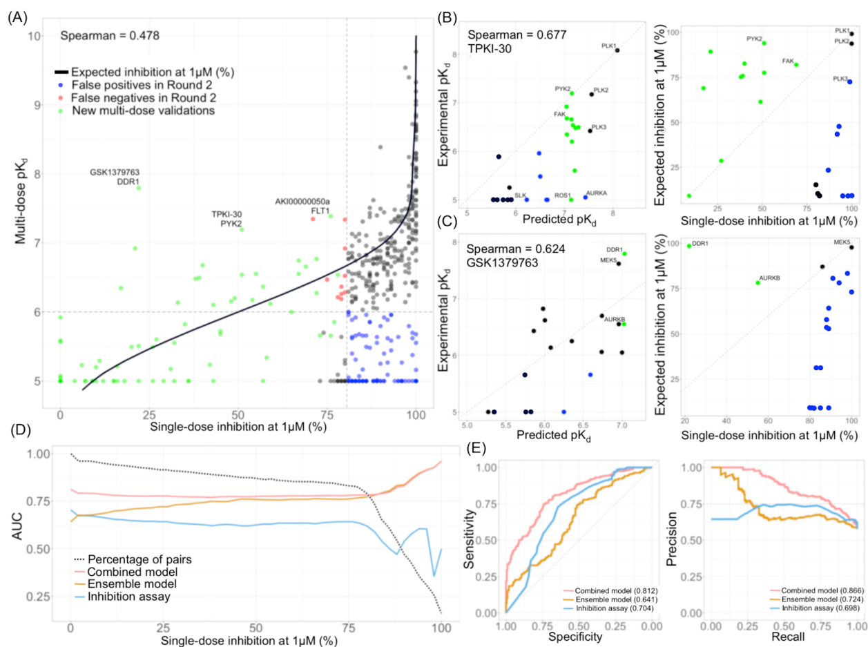
Figure 6. Machine learning-based target predictions. (A) Comparison of single-dose inhibition assay (at 1\mu\text{M} ) against multi-dose K_d assay activities across 475 compound-target pairs (394 Round 2 pairs and 81 additionally profiled pairs). The red points indicate false negatives and blue points false positives when using cut-offs of pK_d = 6 and inhibition=80% among the Round 2 pairs (including 75 pairs with inhibition>80% but that showed no activity in the dose-response assays, i.e, pK_d = 5 ). The green points indicate the new experimental validations based solely on model predictions, regardless of inhibition levels. Both the single-dose and dose-response assays were carried out as competitive binding assays similar to previous studies. 11 The black trace indicates the expected %inhibition rate based on measured pK_d 's, estimated using the maximum ligand concentration of 1\mu\text{M} both for the single-dose and dose-response assays. (B) Multi-dose (left) and single-dose (right) assays for kinases tested with TPKI-30. Green points indicate the new experimental validations based on model predictions, whereas black points come from Round 2 data. Blue points indicate false positive predictions based either on predictive models or single-dose testing. Single-dose testing predicted TPKI-30 to be relatively potent PLK1/2/3 inhibitor, whereas the dose-response testing confirmed it as PLK1 selective. (C) Multi-dose (left) and single-dose (right) assays for kinases tested with GSK1379763. Green points indicate the new experimental validations based on model predictions, whereas black points come from Round 2 data. Blue points indicate false positive predictions based either on predictive models or single-dose testing. (D) Predictive
