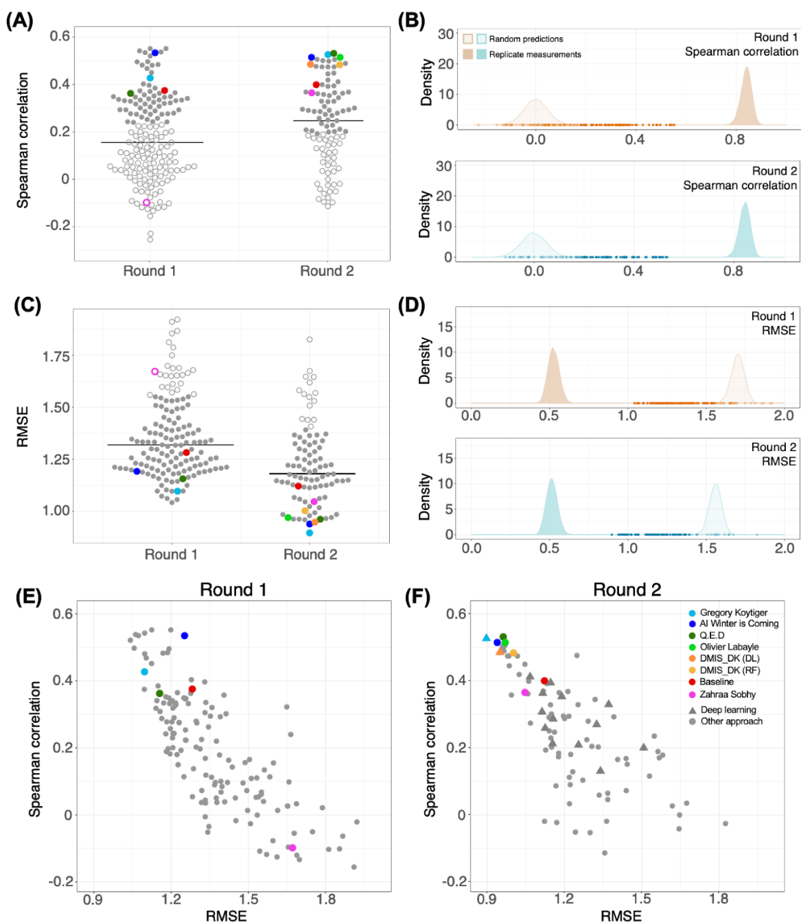
Figure 3. Overall performance of the submissions. (A, C) Performance of the submissions in terms of the two winning metrics in Round 1 ( n=169 ) and Round 2 ( n=99 ). The colors mark the baseline model and top-performing participants in Round 2. The empty circles mark the submissions that did not differ from random predictions. The baseline model 12 remained the same in both of the rounds. (B, D) Distribution of the random predictions (based on 10000 permuted pK_d values) and replicate distributions (based on 10000 subsamples with replacement of overlapping pK_d pairs between two large-scale target activity profiling studies 3,4 ) in Round 1
