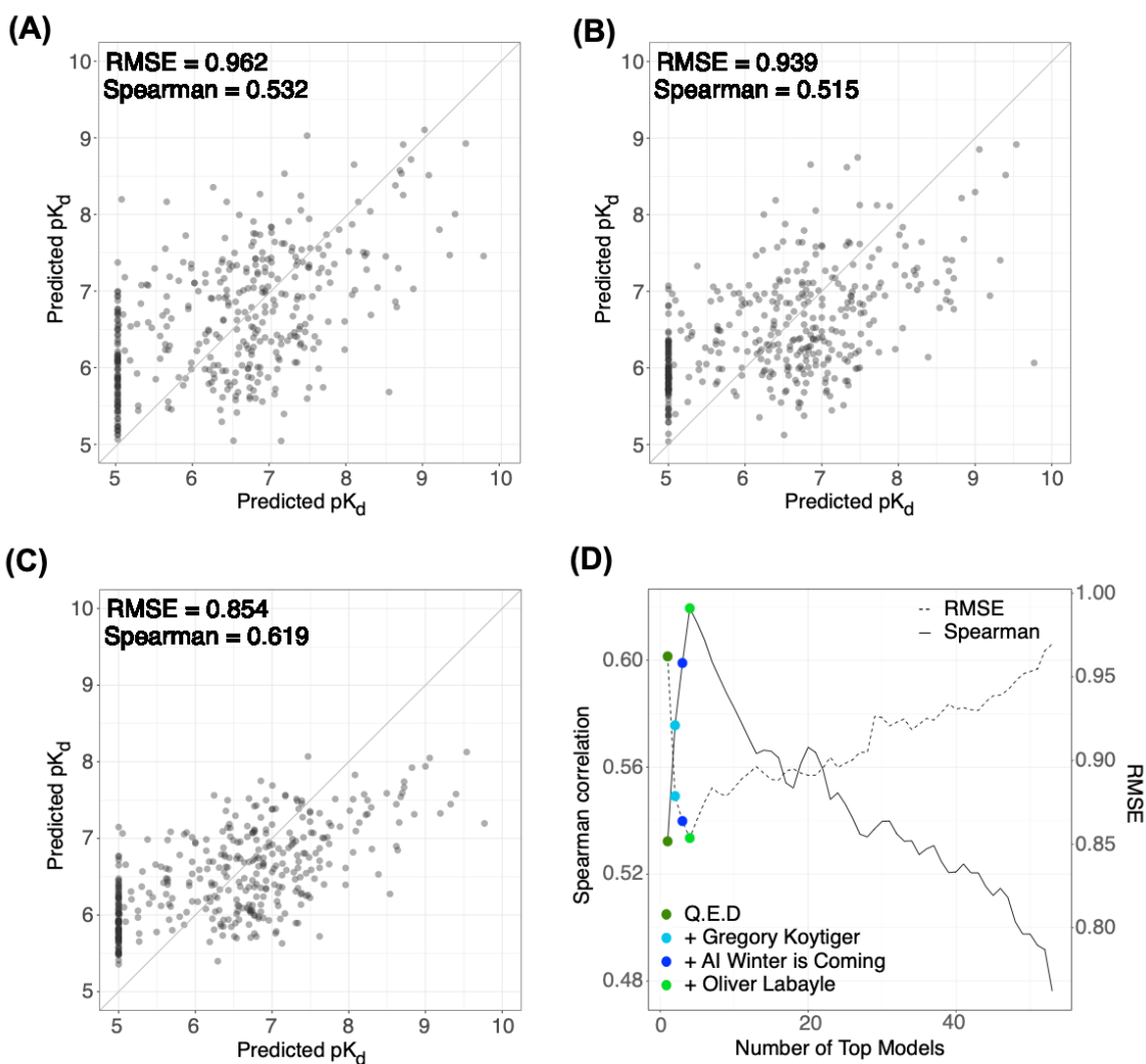
Figure 4. Top-performing models and their ensemble combination. (A) Spearman correlation sub-challenge top-performer in Round 2, Q.E.D. (B) RMSE sub-challenge top-performer in Round 2, AI Winter is Coming. (C) Ensemble model that combines the top four models selected based on their Spearman correlation in Round 2. The points correspond to the 394 compound-kinase pairs between 25 inhibitors and 207 kinases in Round 2. (D) The mean aggregation ensemble model was constructed by adding an increasing number of top-performing models based on their Spearman correlation, until the ensemble correlation dropped below 0.45. The peak performance was reached when aggregating four teams (marked in the legend, see Suppl. Fig. 8 for names of all the teams).
