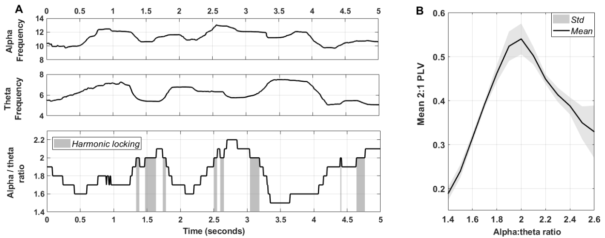
Figure 1. Harmonic locking estimation and its relation to alpha:theta phase synchrony.
