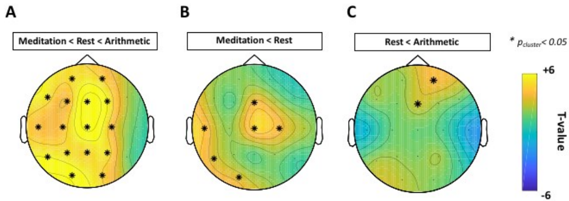
Figure 2. Condition-related differences in alpha:theta harmonic locking (% of time points displaying a 2:1 relationship between alpha and theta oscillations).
