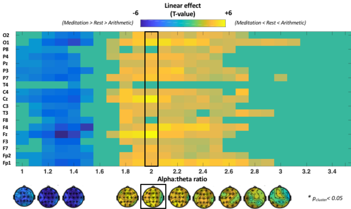
Figure 3. Condition-related differences in the incidence of different alpha:theta cross-frequency relationships (ratios ranging between 1.0 to 3.5). The plot visualizes the estimated linear effect (comparing meditation vs rest vs arithmetic) separately for each electrode (y-axis) and cross-frequency ratio (x-axis). A positive cluster with a widespread spatial distribution was identified for cross-frequency ratios ranging between 1.7 and 3.1, indicating that the incidence (% time points) of this range of ratios was higher in the arithmetic, compared to the rest and meditation condition (i.e. meditation < rest < arithmetic; in warm colours). In addition, negative cluster with a widespread spatial distribution was identified for cross-frequency ratios ranging between 1.0 – 1.5, indicating that for this range of 'lower-end' ratios, the incidence was higher during meditation, compared to rest and arithmetic (i.e. meditation > rest > arithmetic; in cool colours).
