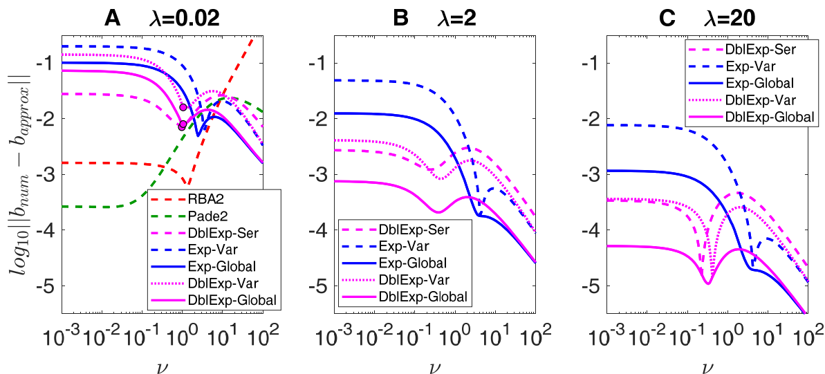
Figure 4. Accuracy comparison of equilibrium nanodomain free buffer concentration approximations obtained by the variational and modified variational (global) methods: Exp-Var ( dashed blue curves ), DbIExp-Var ( dotted magenta curves ), Exp-Global ( blue curves ), and DbIExp-Global ( magenta curves ). For comparison, also shown is the error of DbIExp-Ser ( dashed magenta curves ), and (A) shows the errors of RBA2 ( dashed red curves ) and Pade2 ( dashed green curves ). All panels show the average absolute deviation of free dimensionless buffer concentration (Eq. 29), on base-10 logarithmic scale, as a function of buffer strength parameter \nu ranging from 10^{-3} to 10^2 , for 3 distinct choices of fixed model parameter \lambda : \lambda=0.02 (A), \lambda=2 (B), and \lambda=20 (C), with \eta=1 . Magenta circles in (A) mark values of \nu below which parameter \alpha becomes imaginary for the corresponding DbIExp method. For these smaller value of \nu , the magenta curves in (A) represent the accuracy of buffer concentration given by the real part of Eq. 26.
