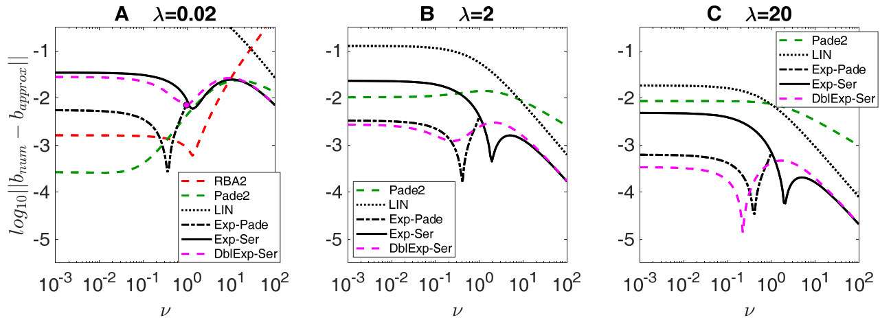
Figure 2. Accuracy comparison of equilibrium free buffer concentration approximations obtained by the series interpolation method: Exp-Ser ( black curves ), Exp-Padé ( dashed black curves ), DblExp-Ser ( dashed magenta curves ), and Padé2 ( dashed green curves ). Also shown is LIN ( dotted black curves ) and RBA2 ( red dashed curve ). RBA2 is only shown in A, since it requires \lambda < 1 . All curves show the error norm given by Eq. 29, on base-10 logarithmic scale, as a function of model parameter \nu ranging from 10^{-3} to 10^2 , for 3 distinct choices of \lambda : \lambda=0.02 (A), \lambda=2 (B), and \lambda=20 (C), with \eta=1 . Since Exp-Padé only yields a solution for \nu < \eta=1 , the corresponding curves terminate at \nu=1 . Magenta circle in (A) indicates the value of \nu below which the exponent parameter \alpha of DblExp-Ser becomes imaginary (this occurs for \lambda < 1.8 ). For smaller value of \nu , the magenta curve in A corresponds to the real part of Eq. 26.
