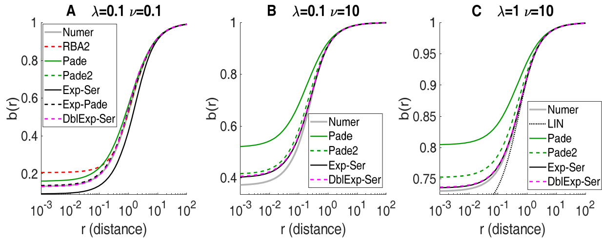
Figure 1. Equilibrium nanodomain buffer concentration \nu approximations obtained using the series interpolation method: 1 st -order Padé ( green ), 2 nd order Padé (Padé2, dashed green ), Exp-Ser ( black ), Exp-Padé, ( dashed black ), and DbExp-Ser ( dashed magenta ). Also shown for comparison is RBA2 (A, dashed red ) and Linear approximation (C, dotted black ). All panels show free dimensionless buffer concentration as a function of distance from the \text{Ca}^{2+} channel, for 3 distinct choices of model parameters \lambda and \nu , as indicated in the panel title, with \eta = 1 . Grey curves show the accurate numerical solution. In (A), DbExp-Ser, Padé2 and Exp-Padé are indistinguishable from the numerical solution on this scale. Note that Exp-Padé does not yield a solution for \nu > \eta = 1 (B,C). In (A), DbExp-Ser curve shows the real part of Eq. 26.
