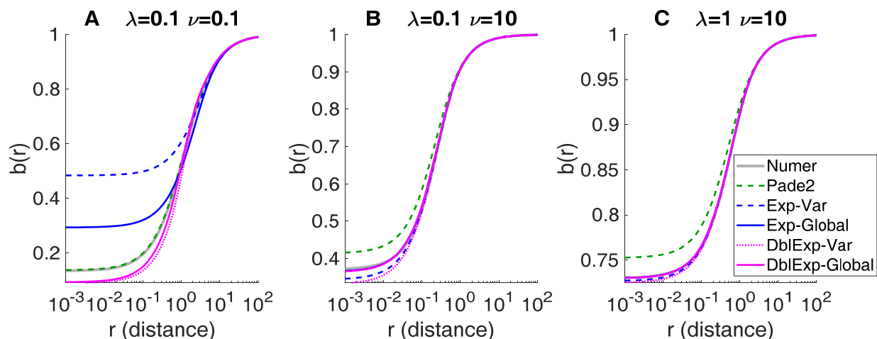
Figure 3. Comparison of equilibrium buffer concentration approximants obtained using the variational and the modified variational (global) methods: Exp-Var ( dashed blue curves ), DbIExp-Var ( dotted magenta curves ), Exp-Global ( blue curves ), and DbIExp-Global ( magenta curves ). Padé2 is also shown for comparison ( dashed green curves ). All panels show the free dimensionless buffer concentration as a function of distance from the \text{Ca}^{2+} channel, for 3 distinct choices of model parameters \lambda and \nu , with \eta=1 . Grey curves show the accurate numerical solution. In (A), the real part of DbIExp-Var and DbIExp-Global is shown. In (B) and (C), the curves for Exp-Global and DbIExp-Global overlap the numerical solution.
