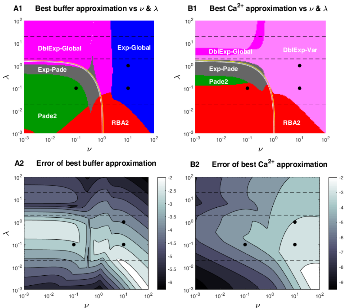
Figure 6. Comparison of parameter regions where a given approximant outperforms the rest in estimating (A1) free buffer and (B1) \text{Ca}^{2+} concentration in the (\nu, \lambda) parameter plane, according to the error measures given by Eqs. 28 and 36. In all panels, \eta=1 . Colors indicate parameter region of best performance for each approximant: Padé2 (green), RBA2 (red), Exp-Padé (gray), DbExp-Var (pink), DbExp-Global (magenta), Exp-Global (blue). Black circles corresponds to parameter values in Figs. 1,3, and dashed lines corresponds to the parameter sweep curves in Figs. 2,4-6. Thin light semi-circular curves indicate the boundaries inside of which the exponent parameters \alpha in the DbExp-Var and DbExp-Global methods becomes imaginary ( \alpha is always real outside of the region marked by these curves, for \nu > 1 and \lambda > 1.8 ). Lower panels show the smallest error in estimating buffer (A2) and \text{Ca}^{2+} (B2) concentrations achieved using the optimal approximants shown in top panels. The grayscales in A2 and B2 indicate the log-10 error values given by Eqs. 28 and 36, respectively
