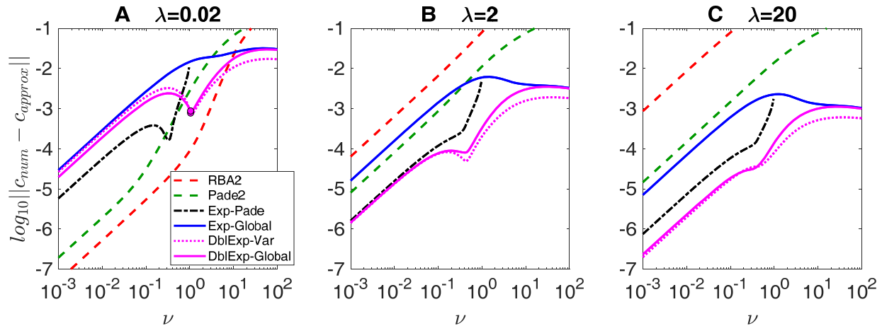
Figure 5. Accuracy comparison of equilibrium nanodomain \text{Ca}^{2+} concentration estimation by select optimal approximations (methods with smallest error): RBA2 ( red dashed curves ), Padé2 ( dashed green curves ), Exp-Padé ( dot-dashed black curves ), Exp-Global ( blue curves ), DblExp-Global ( magenta curves ), and DblExp-Var ( dotted magenta curves ). All panels show average absolute deviation of free dimensionless \text{Ca}^{2+} concentration (Eq. 36), on base-10 logarithmic scale, as a function of buffering strength parameter \nu ranging from 10^{-2} to 10^2 , for 3 distinct choices of diffusivity parameter \lambda : \lambda=0.02 (A), \lambda=2 (B), and \lambda=20 (C), with \eta=1 . Curves for Exp-Padé ( dashed black curves ) terminate at \nu=1 .
