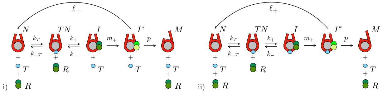
FIG. 1. Kinetic proofreading scheme for chromatin remodeling with nucleosome ( N ), pioneer transcription factor ( T ), remodeler ( R ). Two scenarii are shown: i) early pTF unbinding; ii) late pTF unbinding. In case i), I denotes the remodeler-nucleosome complex and I^* the activated complex; M is the mobile nucleosome. In case ii) I and I^* stand for the corresponding remodeler-nucleosome-pTF complexes. The translocation step with rate p is shown to ultimately lead to remodeler dissociation; this step is in general processive.
