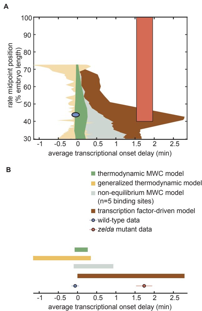
Figure S9: Exploration of state space. (A) Two-dimensional state-space exploration, showing the extents of state space of the wild-type (blue) and zelda - (red) data as well as of various models explored in the main text. (B) One-dimensional state-space exploration, created by projecting the two-dimensional state space in (A) for rate midpoint values between 40% and 100% onto the x-axis corresponding to the average t_{on} delay. Areas covered by the experimental data represent the standard error of the mean.
