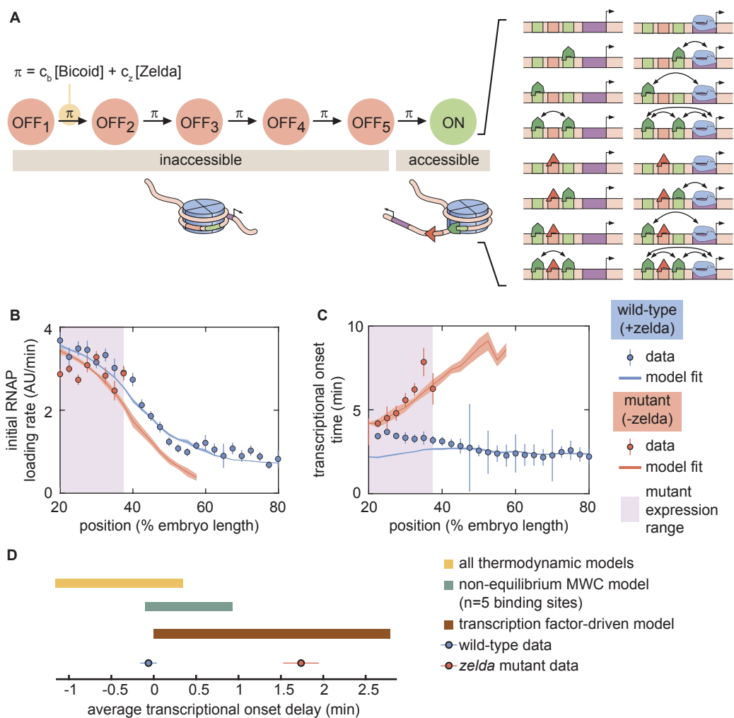
Figure 7: A model of transcription factor-driven chromatin accessibility is sufficient to recapitulate hunchback transcriptional dynamics. (A) Overview of the proposed model, with five ( m = 5 ) effectively irreversible Zelda and/or Bicoid-mediated intermediate transitions from the inaccessible to the accessible states. (B,C) Experimentally fitted (B) initial RNAP loading rates and (C) t_{on} for wild-type and zelda - embryos using a single set of parameters and assuming six Bicoid binding sites. (D) The domain of average t_{on} delay covered by this transcription factor-driven chromatin accessibility model (brown rectangle) is much larger than those of the generalized thermodynamic model (yellow rectangle) and the non-equilibrium MWC models (green rectangle), and easily encompasses both experimental datasets (points). (B-D, error bars represent standard error of the mean over multiple embryos).
