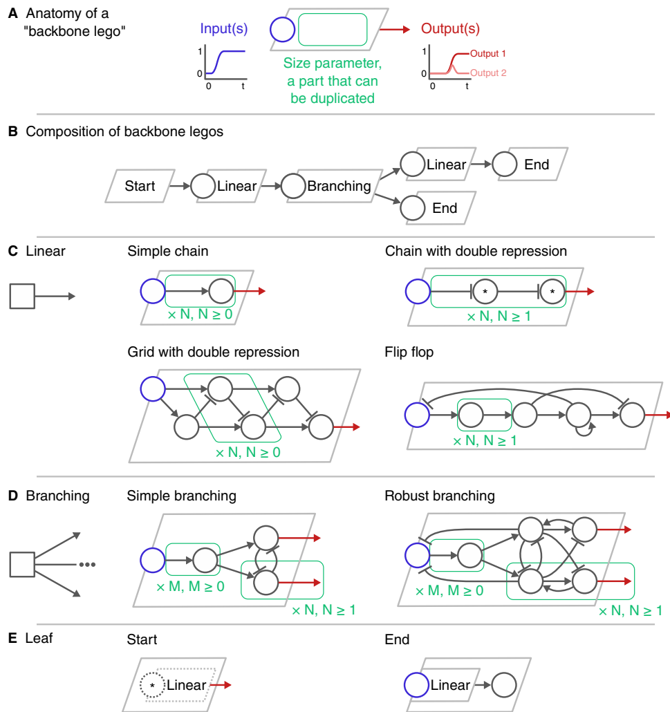
Figure 9: Reusable regulatory building blocks that can be used to construct GRNs that result in dynamic processes following an expected pattern. A: Each building block contains genes which serve as inputs that can be regulated by external transcription factors. The connections inside the building block transform the input signal in a particular way and has one or more output interactions of which the targets are not yet determined. B: By connecting multiple building blocks together, a backbone of regulatory modules can be formed. C: dyngen offers several variations of linear building blocks which allow for differing regulatory mechanisms. D: A branching module will upregulate the expression of just one of the output interactions. Two variations are given of which the simple variant is more prone to reprogramming events in comparison to the robust branching module. E,F: These components allow to specify the beginning (no inputs) and end (no outputs) of the backbone.
