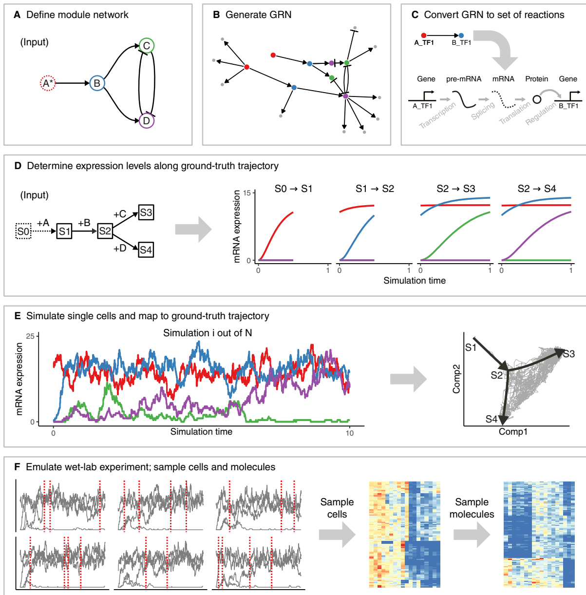
Figure 7: The workflow of dyngen is comprised of six main steps. A: The user needs to specify the desired module network or use a predefined module network. B: Each gene in a module is regulated by one or more transcription factors from the upstream module. Additional target genes are generated. C: Each gene regulatory interaction in the GRN is converted to a set of biochemical reactions. D: Along with the module network, the user also needs to specify the backbone structure of expected cell states. The average expression of each edge in the backbone is simulated by activating a restricted set of genes for each edge. E: Multiple Gillespie SSA simulations are run using the reactions defined in step C. The counts of each of the molecules at each time step are extracted. Each time step is mapped to a point in the backbone. F: The molecule levels of multiple simulations are shown over time (left). From each simulation, multiple cells are sampled (from left to middle). Technical noise from profiling is simulated by sampling molecules from the set of molecules inside each cell (from middle to right).
