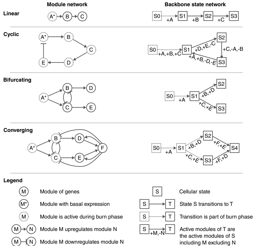
Figure 8: Example module networks.
