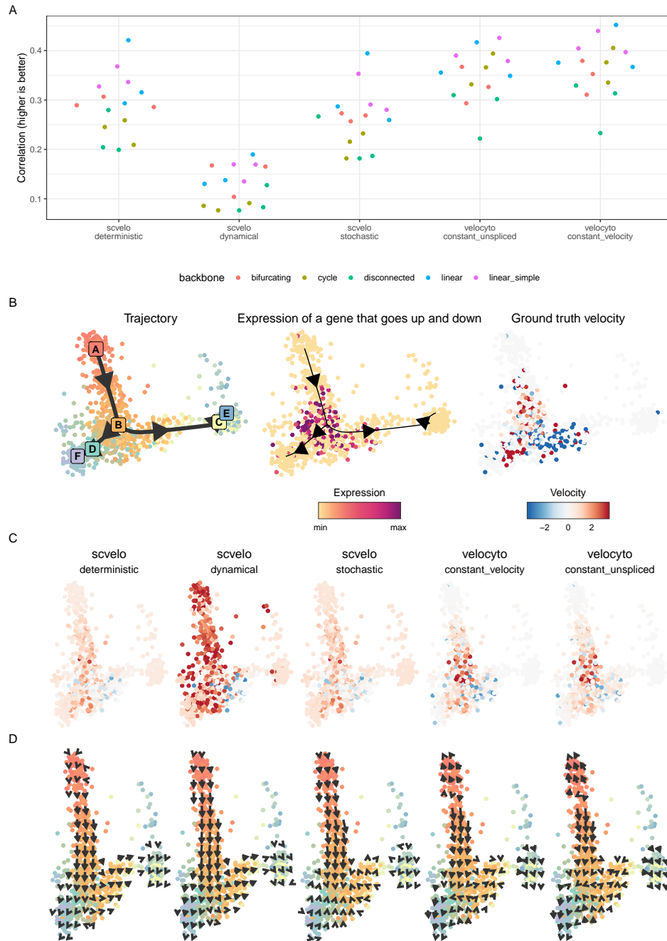
Figure 4: dyngen allows benchmarking of RNA velocity methods. A: We tested five different methods and parameter settings for the estimation of RNA velocity on datasets with varying backbones (colours). Overall, the velocityto method with the constant velocity assumption performed the best overall. B: An example bifurcating dataset, with as illustration the expression and ground truth velocity of a gene that goes up and down in the trajectory. C: The RNA velocity estimates of the different methods. D: The embedded RNA velocity of the different methods.
