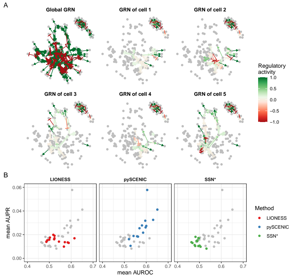
Figure 5: dyngen allows benchmarking Cell-specific Network Inference (CSNI) methods. A: A cell is simulated using the global gene regulatory network (GRN, top left). However, at any particular state in the simulation, only a fraction of the gene regulatory interactions are active. B: CSNI methods were executed to predict the regulatory interactions that are active in each cell specifically. Using the ground-truth cell-specific GRN, the performance of each method was quantified on 14 dyngen datasets.
