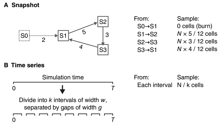
Figure 11: Two approaches can be used to sample cells from simulations: snapshot and time-series.
